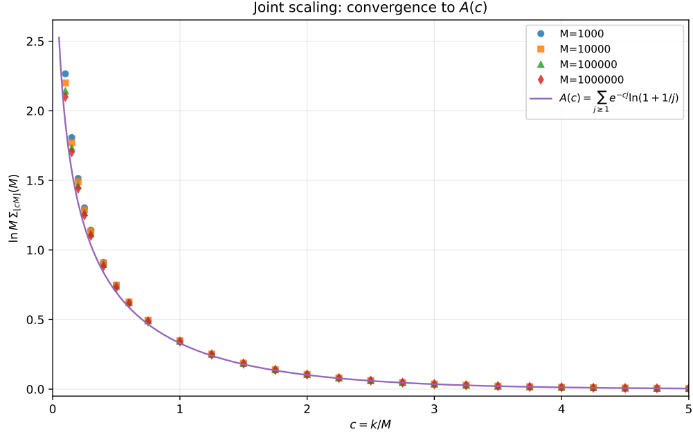
Figure 2: Joint scaling regime k = \lfloor cM \rfloor . Points show \ln M \cdot \Sigma_{\lfloor cM \rfloor}(M) , evaluated deterministically by direct prime summation in double precision (no Monte Carlo), at M \in \{10^3, 10^4, 10^5, 10^6\} . Solid curve: A(c) = \sum_{j \geq 1} e^{-cj} \ln(1 + 1/j) , evaluated by adaptive truncation of the positive series when the next term is below 10^{-17} .
