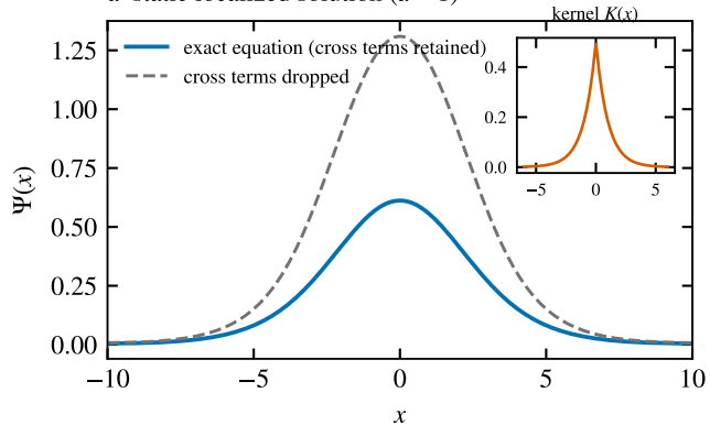
a static localized solution ( d = 1 )
