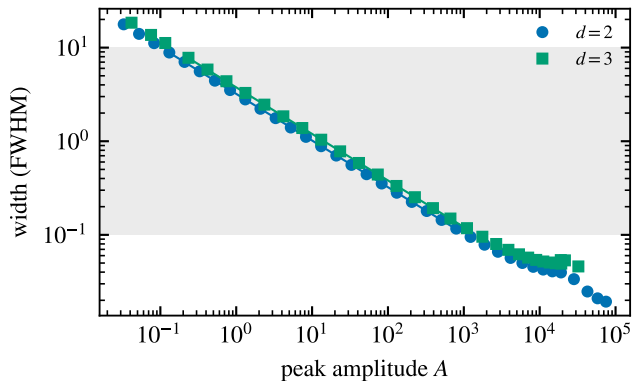
d envelope states: w \propto A^{-1/2} in the window
