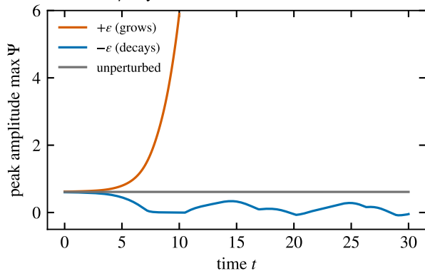
c full \Psi - \phi_0 dynamics from the static solution
