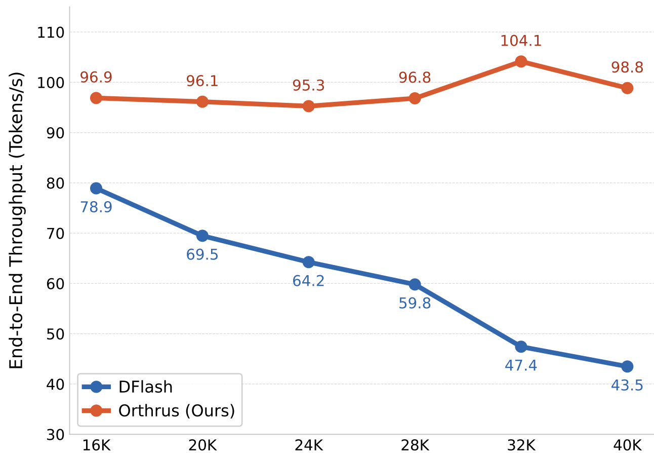
Long Context Throughput Scaling
