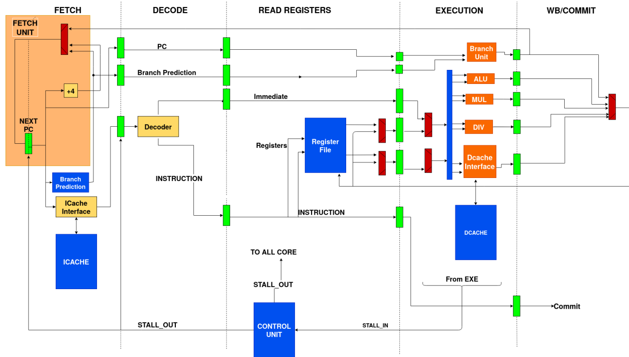
Figure 3.1: Top-level organization of the Sargantana datapath
