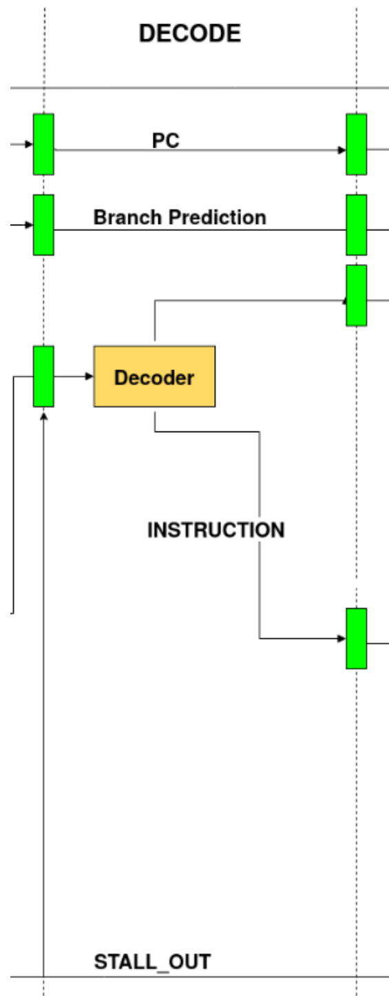
Figure 6.2: Detailed signal view of the Decode stage
