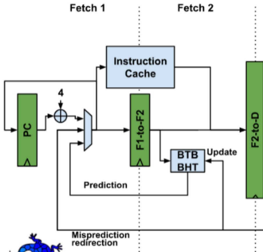
Figure 4.1: Fetch Stage 1 and Fetch Stage 2 organization
