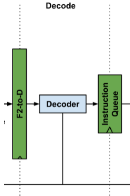
Figure 6.1: Decode stage: F2-to-D → Decoder → Instruction Queue
