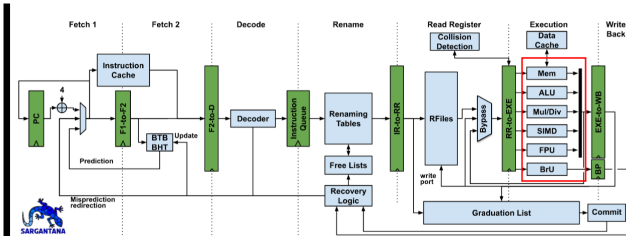
Figure 11.2: Result collection: completed results from the highlighted execution units feed the writeback stage
