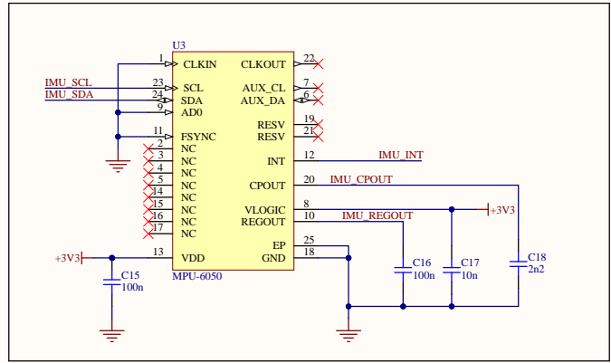
Interial Measurement Unit (MPU-6050)
