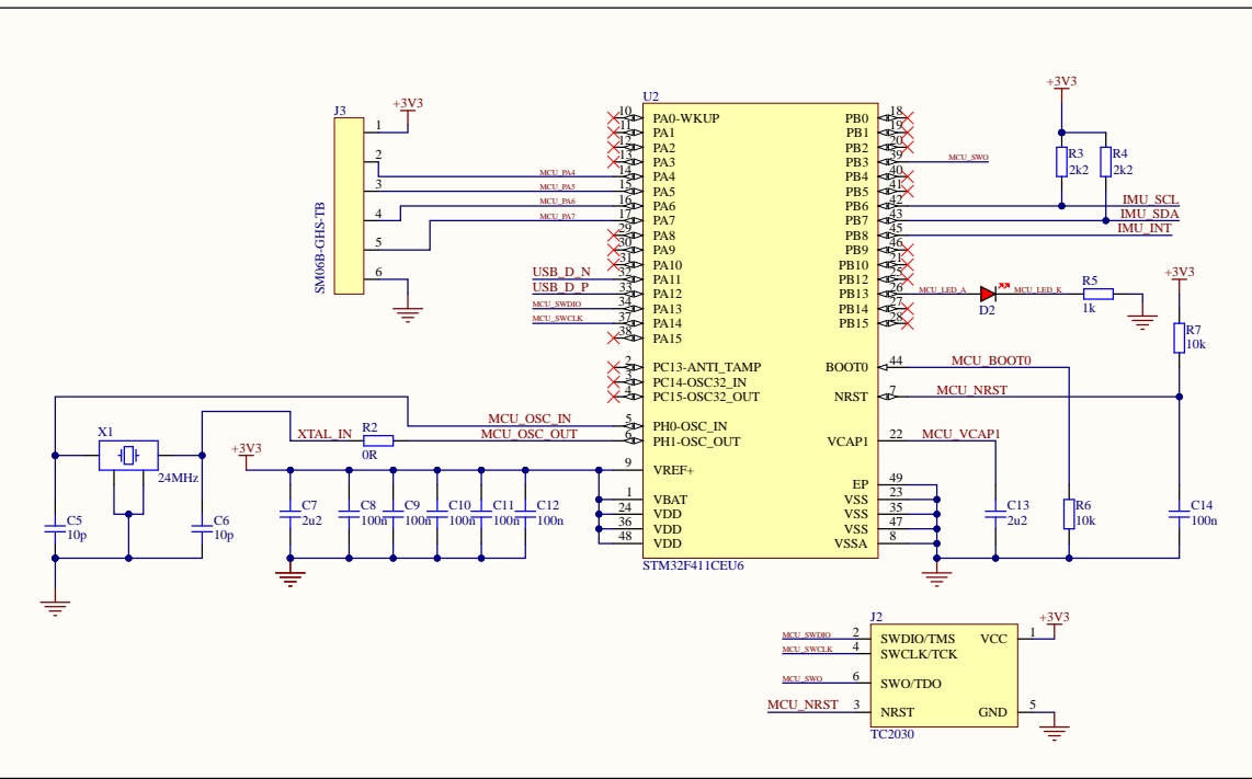
Microcontroller(STM32f4)
