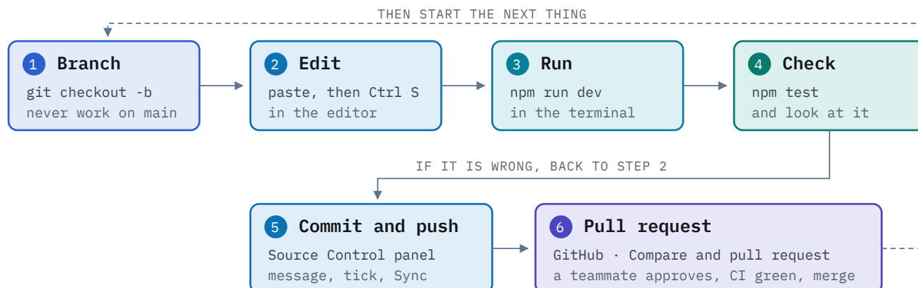
Figure 10. The loop. Every code block in Parts 2 and 3 is step 2; every “check it works” box is step 4.
