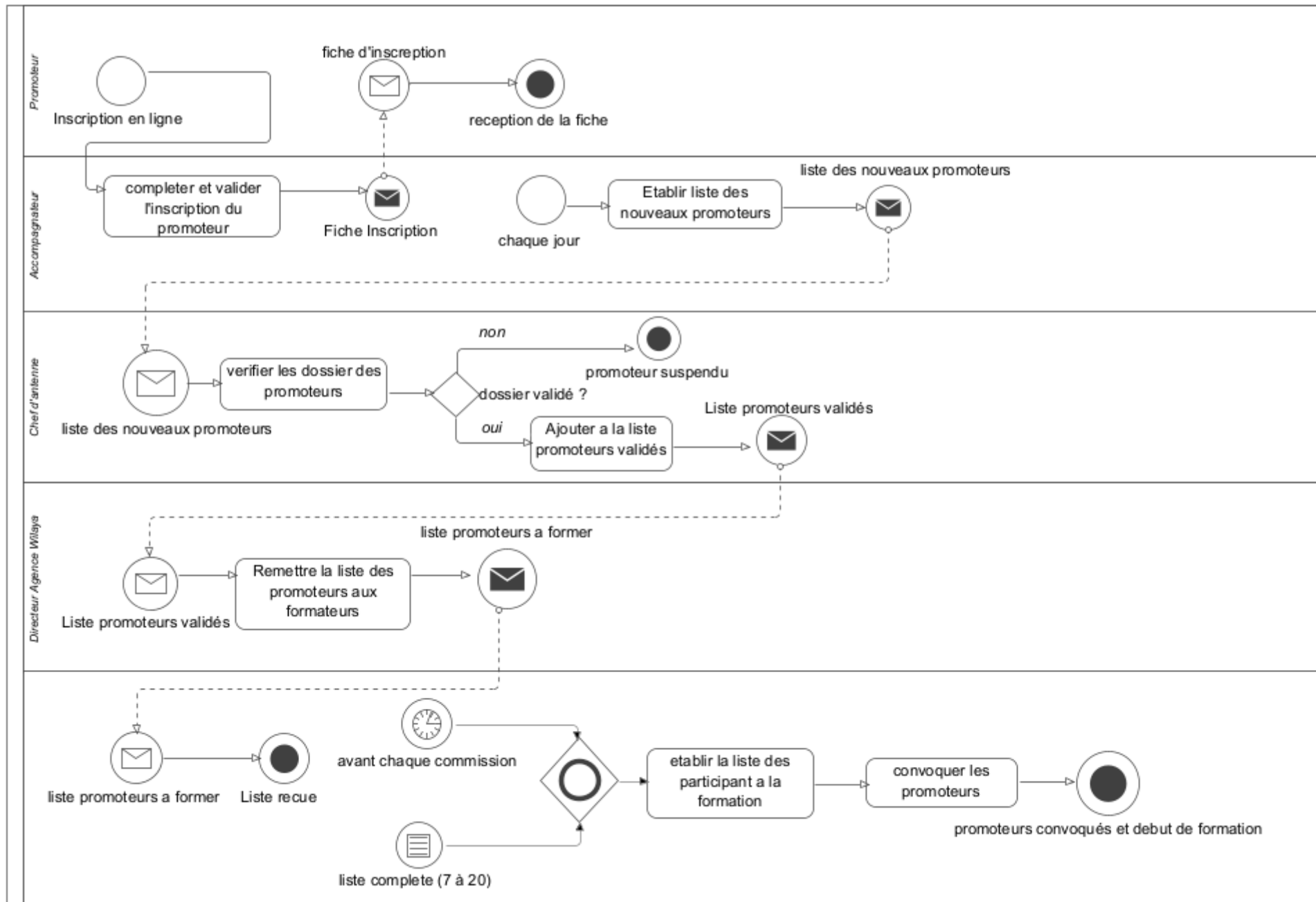
Figure 1.3 BPMN
