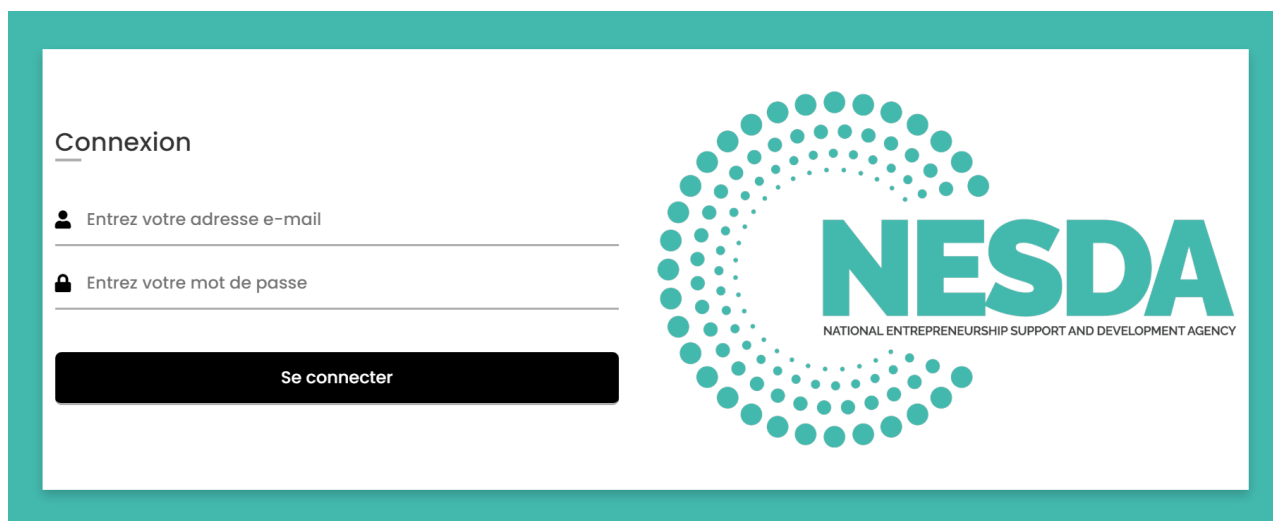
Figure 3.1 interface d'authentification
