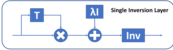
Fig. 1. Single inversion layer for inferring \mathbf{G}_k^{(i)} from \mathbf{F}_{k-1} .
