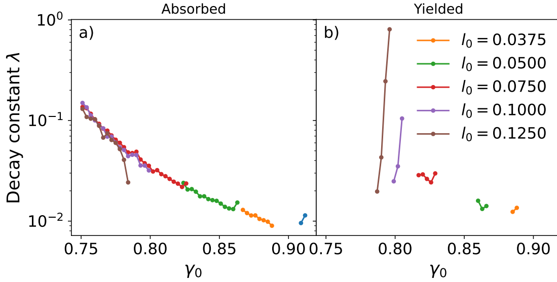
Figure 3.8. Decay constants \lambda characterising the exponential tails of the survival functions shown in Fig. 3.7. For each annealing parameter l_0 and strain amplitude, \lambda is obtained by fitting the large- C^* regime to S(C^*) \sim \exp(-\lambda C^*) . Results are shown separately for absorbing and yielding trajectories.
