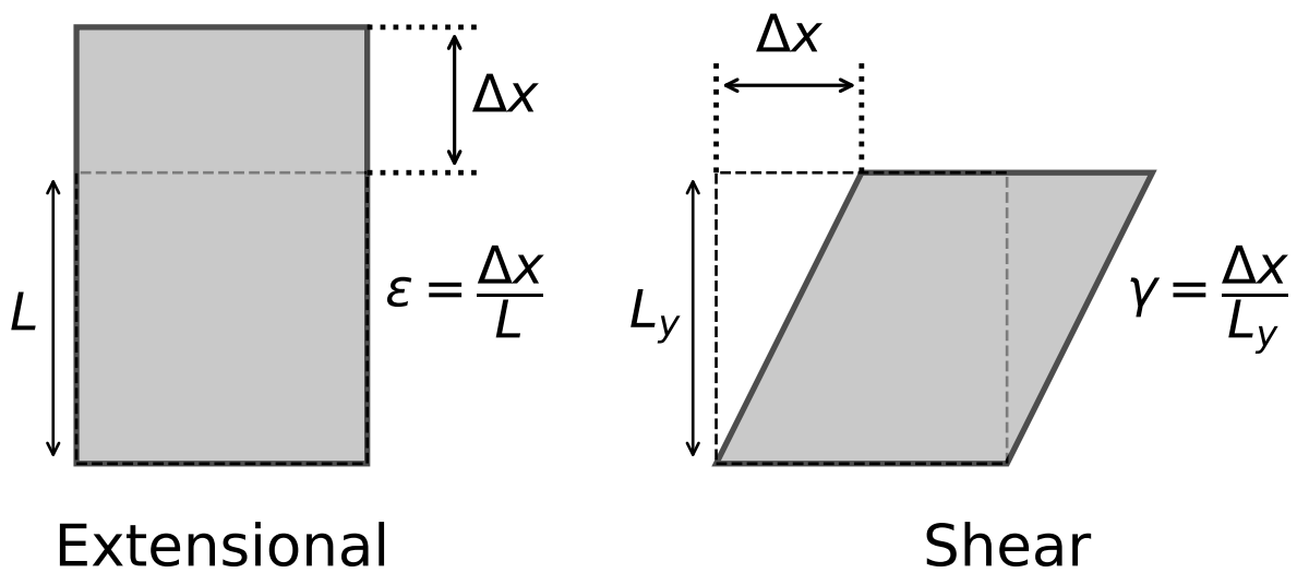
Figure 1. Illustration of the two fundamental strain modes in 2D: extensional strain \epsilon , where the element changes length, and shear strain \gamma \equiv \gamma_{xy} , where the element changes shape through angular distortion. The dashed lines denote the material's undeformed configuration, while the solid lines indicate its deformed state.
