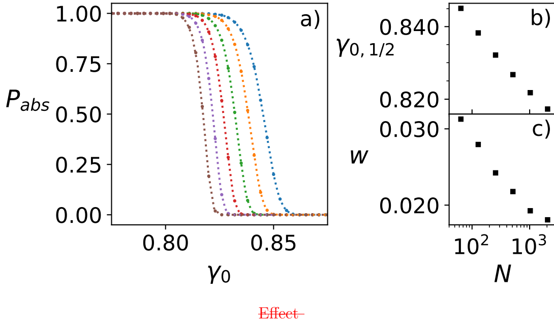
Figure 3.11. Finite-size dependence of system size N the transition between absorption and yielding at fixed parameters l_0 = 0.075 and l_w = 0.02 .
