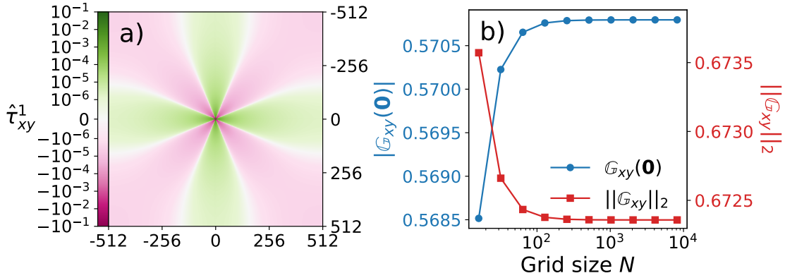
Figure 3.1. a) Stress redistribution \tau_{xy}^1 resulting from a point stress perturbation S_{xy} = 1 in 2D b) Convergence Finite-system-size convergence of the magnitude of the value at the origin \mathbb{G}_{xy}(\mathbf{0}) , |\mathbb{G}_{xy}(\mathbf{0})| , and the norm \|\mathbb{G}_{xy}\|_2 with increasing grid size N .
