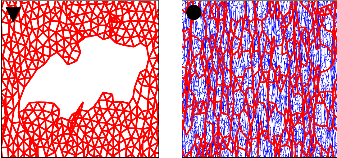
(a) Initiation of a macroscopic crack in a stretched single sacrificial network, which will result in a catastrophic material failure.
