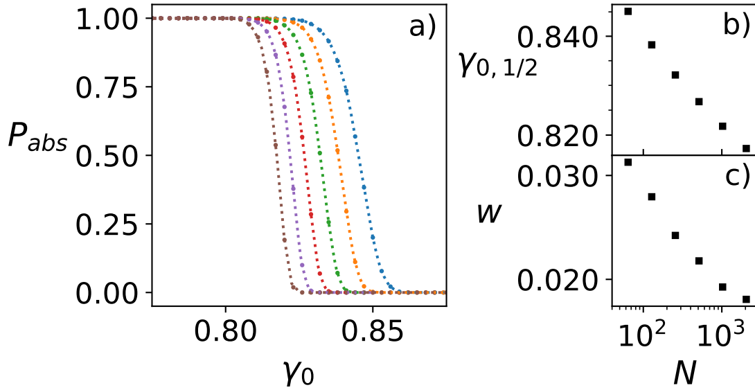
Figure 3.11. Finite-size dependence of system size N the transition between absorption and yielding at fixed parameters l_0 = 0.075 and l_w = 0.02 .
