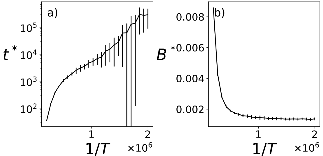
Figure 4.7. Failure time t^* a) and the corresponding fraction of broken bonds B^* b) as a function of temperature T at low imposed strain \gamma_0 = 0.01 . Parameters: E = 5.025 \times 10^{-5} and N = 64,000 .
