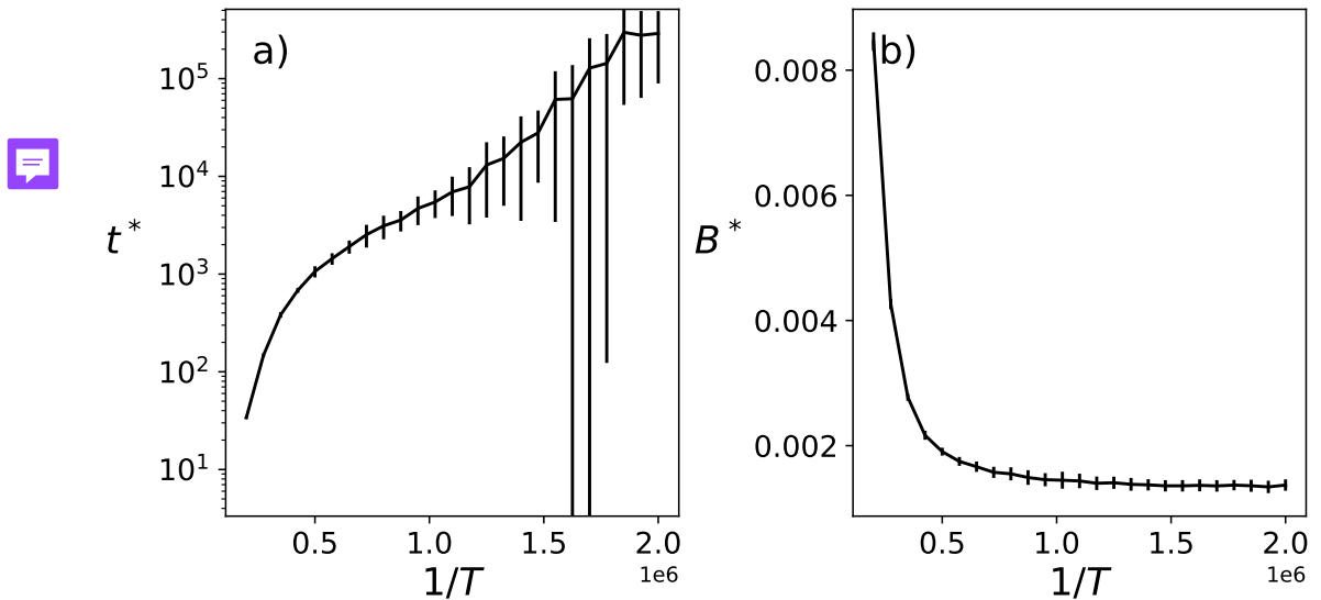
Figure 4.7. Failure time t^* a) and the corresponding fraction of broken bonds B^* b) as a function of temperature T at low imposed strain \gamma_0 = 0.01 . Parameters: E = 5.025 \times 10^{-5} and N = 64,000 .
