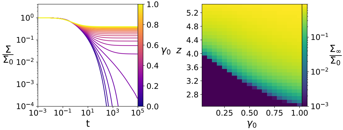
Figure 4.2. Stress relaxation of networks after a step strain of amplitude \gamma_0 .
