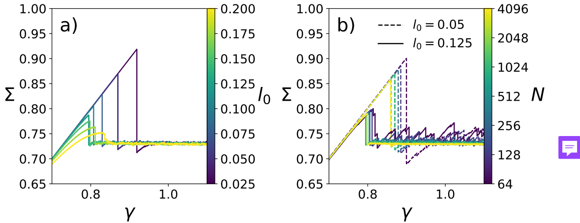
Figure 3.3. Stress-strain curves of the lattice elastoplastic model under shear startup. a) Responses for a lattice size N \times N = 1024 \times 1024 , with decreasing levels of sample annealing in curves downwards: l_0 = 0.025, 0.05, 0.075, \dots, 0.2 . b) Finite-size dependence for two different annealing levels l_0 = 0.05 (dashed curves) and l_0 = 0.125 (solid curves) for system sizes N = 64, 128, 256, 512, 1024, 2048, 4096 .
