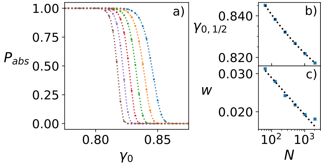
Figure 3.11. Effect of system size N at fixed parameters l_0 = 0.075 and l_w = 0.02 .
