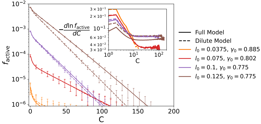
Figure 3.15. Comparison of the decay of the number of active elements in the system with predictions from simplified models. Curves show the mean fraction of active elements f_{\text{active}} averaged over 1,000 samples, and are plotted while at least 500 samples remain active. Results from the full elastoplastic model (EP model) are compared with those from the dilute model. Inset: The logarithmic decay gradient, -d \ln f_{\text{active}} / dC , for the same curves. Locations of curves are indicated on Fig. 3.16.
