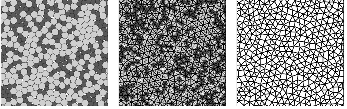
Figure 2.7. Steps for generating a packing-derived network from 400 soft disks at \phi = 1 . Left: A bidisperse disk packing with a radius ratio of 1 : 1.4 in an energy-minimised state. Middle: Network bonds defined from the contact network of overlapping disks. Right: Disks removed, leaving only the bonds and nodes of the network.
