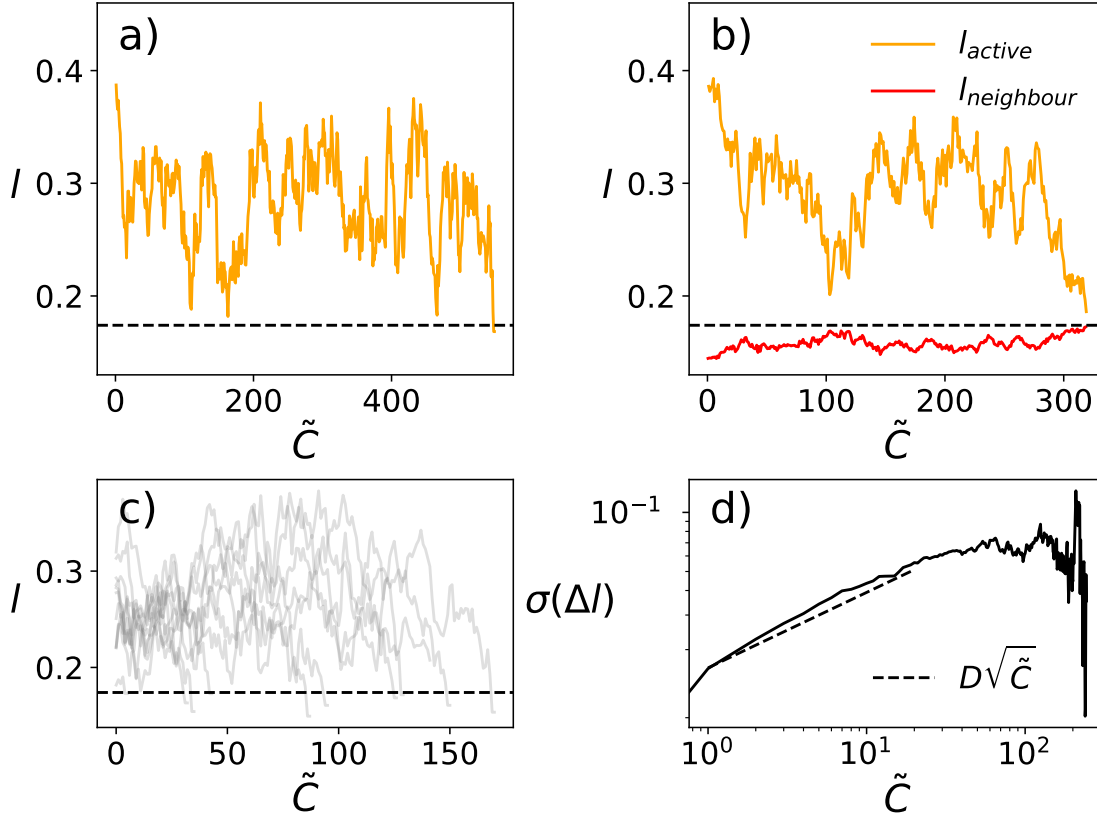
Figure 3.14. Stroboscopic evolution of element strain l measured at the start of each cycle. \tilde{C} indicates the number of cycles after the random walk has begun.
