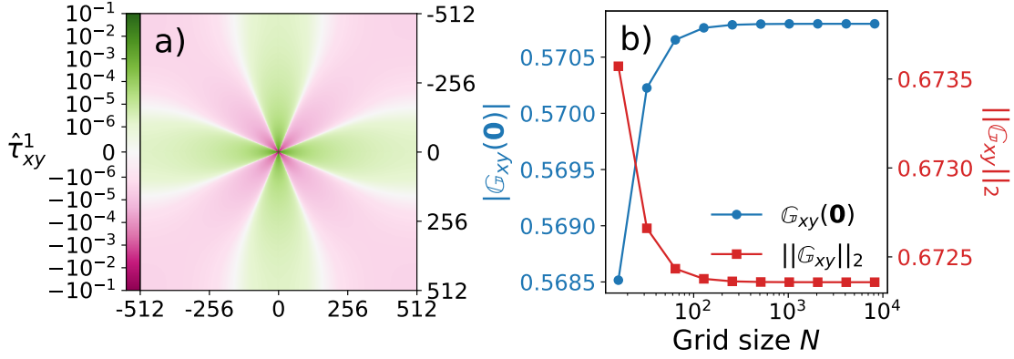
Figure 3.1. a) Stress redistribution \tau_{xy}^1 resulting from a point stress perturbation S_{xy} = 1 in 2D b) Convergence of the value at the origin G_{xy}(\mathbf{0}) and norm \|G_{xy}\|_2 with increasing grid size N .
