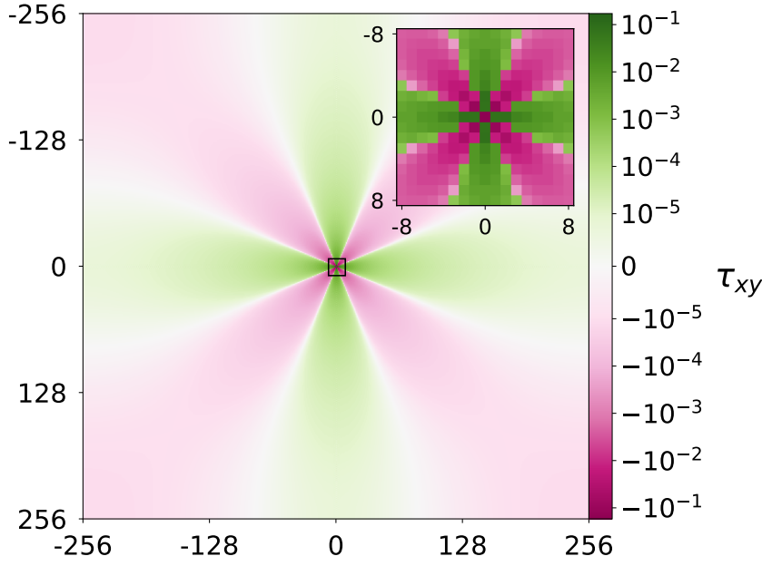
Figure 2.5. Quadrupolar redistribution of shear stress \tau_{xy} in two dimensions, after a single local plastic event in a system with \mu = 1 . The system is initialised with \tau_{xy} = 0 everywhere; one central element is then yielded and set to \tau_{xy} = -1 , after which mechanical equilibrium is enforced. The main panel shows the full N_x \times N_y = 512 \times 512 propagator, and the inset shows the central 17 \times 17 region around the propagator.
