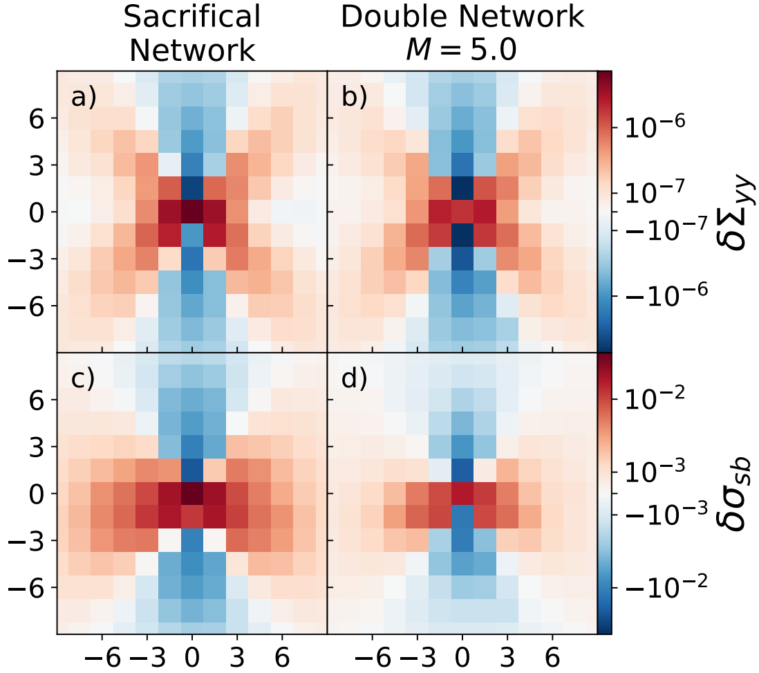
Figure 5.5. Stress propagation to neighbouring sacrificial bonds from the breakage of a sacrificial bond at the origin. We display each quantity for the case of a single sacrificial network in the left column and a double network with M = 5 in the right column. In the double network cases, we take \mu_m = 0.2 . Each quantity is averaged over all sacrificial bonds at each grid square.
