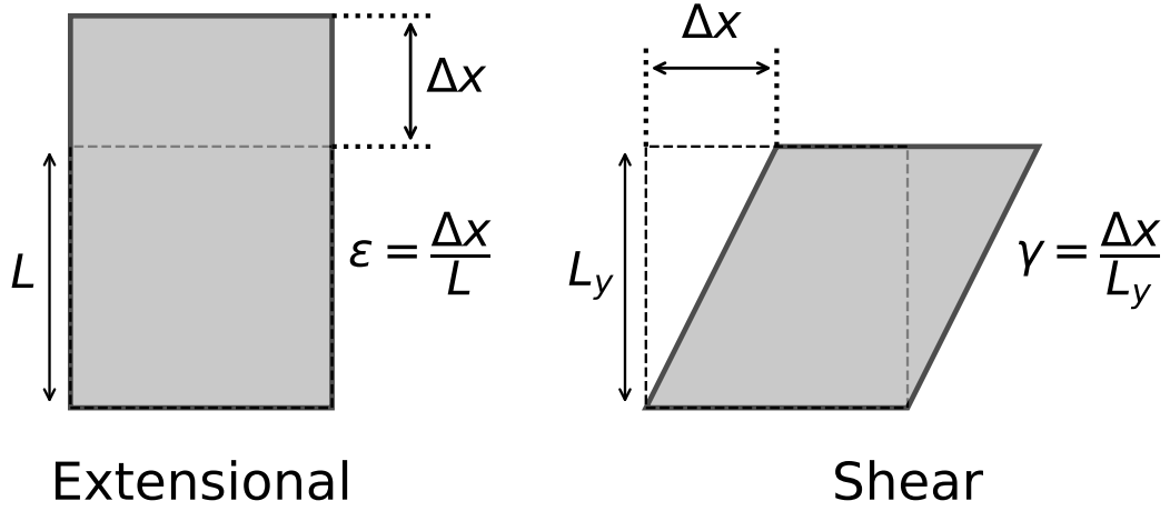
Figure 2.1. Illustration of the two fundamental strain modes in 2D: extensional strain \epsilon , where the element changes length, and shear strain \gamma , where the element changes shape through angular distortion. The dashed lines denote the material's undeformed configuration, while the solid lines indicate its deformed state.
