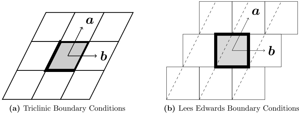
Figure 2.9. Illustration of two equivalent boundary conditions used in simulations to apply macroscopic stress to a system.
