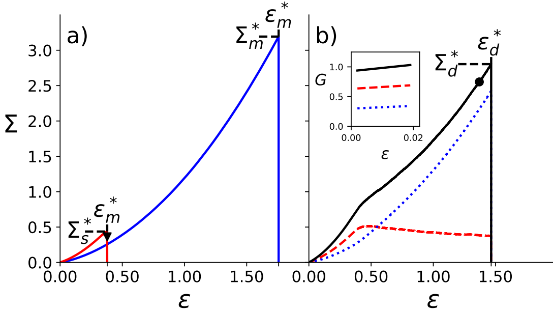
Figure 5.2. Stress-strain curves of a packing-derived network. \Sigma is the yy component of the virial stress tensor defined in section 2.4.7 and \epsilon is the engineering strain along the y direction defined as \epsilon = L_y/L_{y,0} - 1 .
