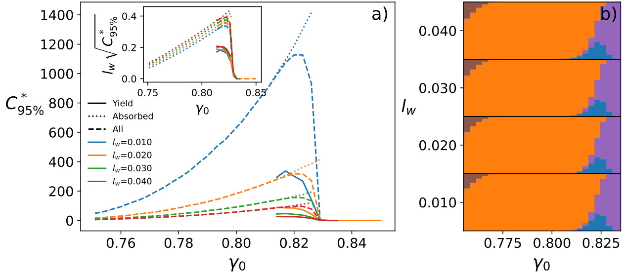
Figure 1.5. Effect of changing the width l_w of the post-hop distribution, with the annealing parameter fixed at l_0 = 0.075 and system size N = 1024 .
