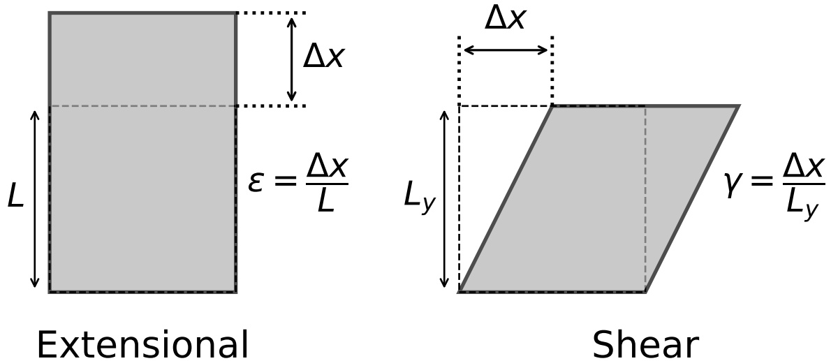
Figure 1. Illustration of the two fundamental strain modes in 2D: extensional strain \epsilon , where the element changes length, and shear strain \gamma \equiv \gamma_{xy} , where the element changes shape through angular distortion. The dashed lines denote the material's undeformed configuration, while the solid lines indicate its deformed state.
