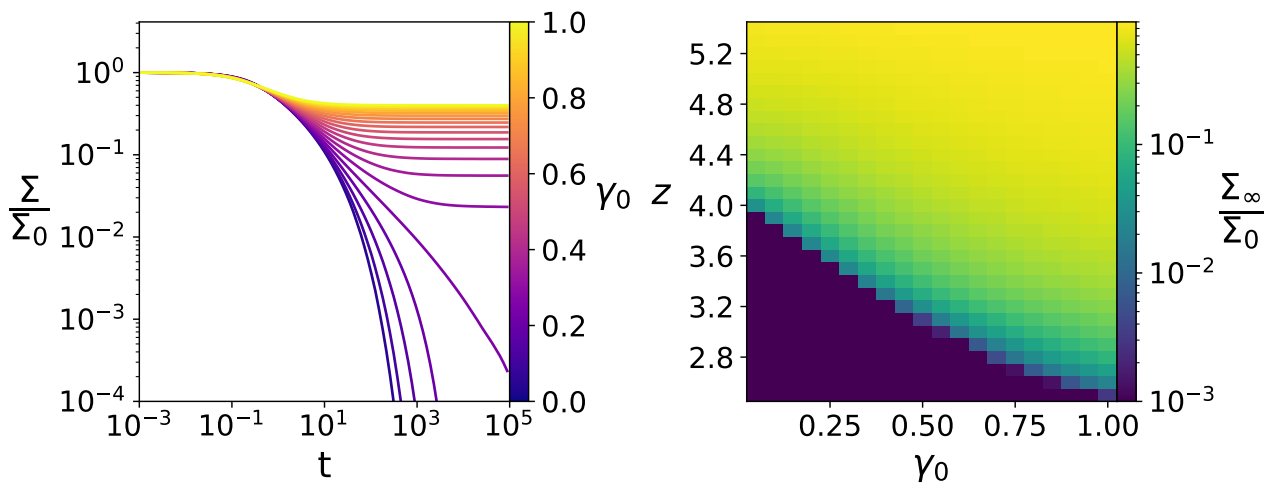
Figure 1.10. Stress relaxation of packing-derived networks pruned to the specified average coordination z after a step strain of amplitude \gamma_0 .
