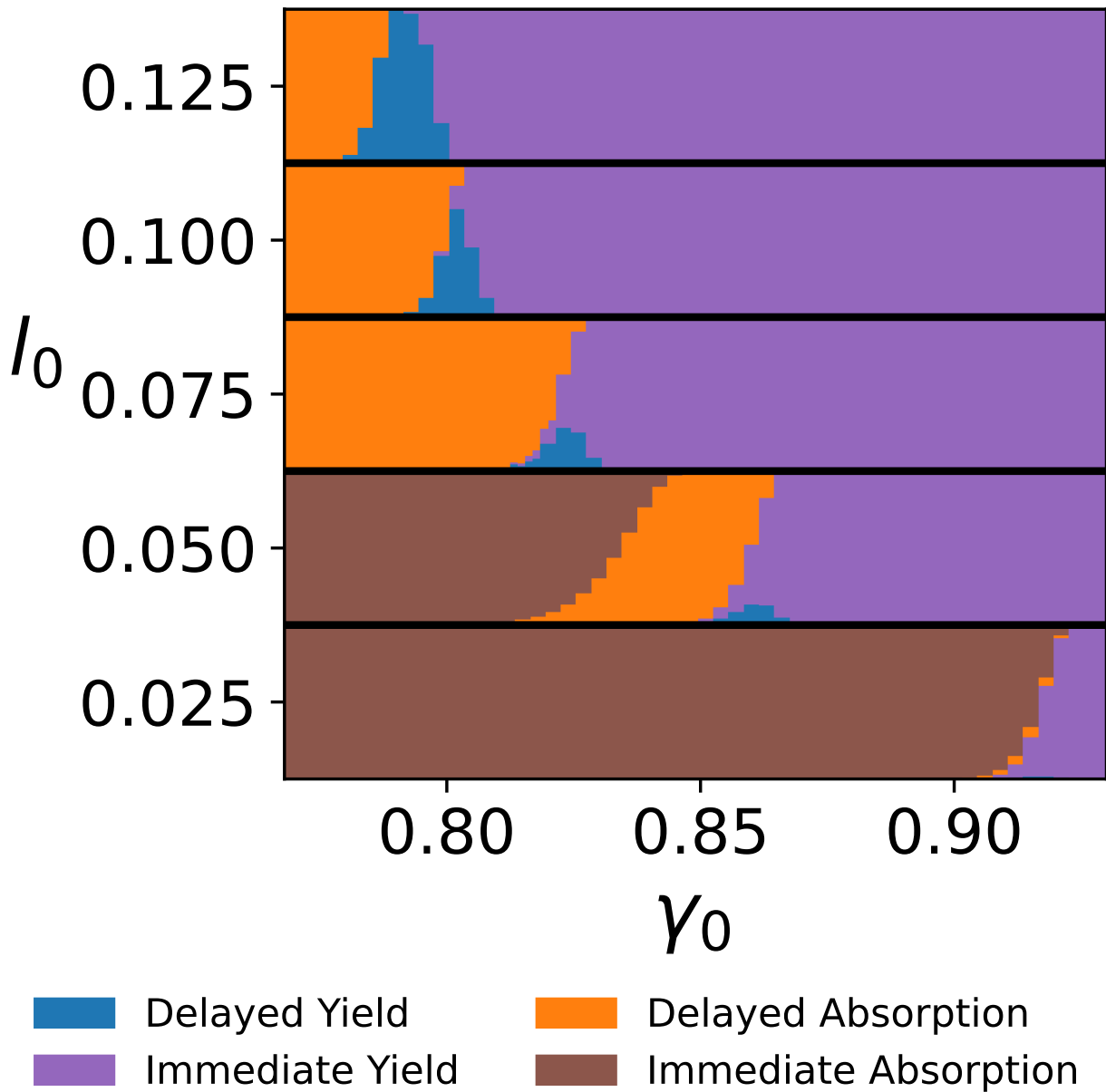
Figure 1.2. Distribution of simulation end states as a function of imposed strain. For each strain amplitude on the x -axis, stacked bars show the fraction of realisations classified according to two binary criteria: whether failure occurs on the first cycle (immediate) or at later cycles (delayed), and whether the system ultimately becomes absorbed or yields. Results are shown for five values of the annealing parameter l_0 (arranged vertically), with smaller l_0 corresponding to better-annealed samples. Each bar represents the statistical outcome over all simulations at the corresponding (\gamma, l_0) pair. For each value of \gamma_0 and l_0 , the distributions are made up of at least 10,000 samples Each parameter combination contains more than 2,500 independent realisations, each sample generated with a different value of the random-number-random-number seed; the exact ensemble sizes are reported in ??.
