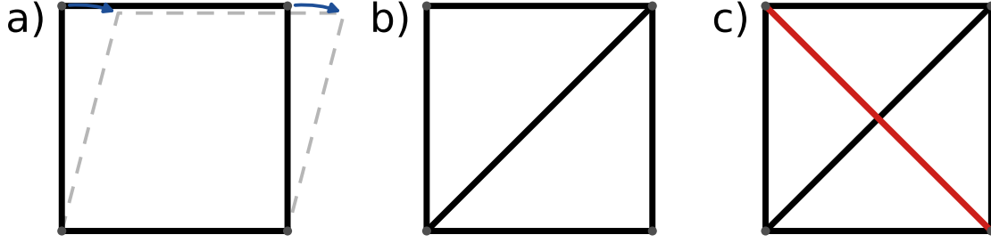
Figure 3. Illustration of Maxwell counting for a connected central-force network with N = 4 nodes in two dimensions. Removing two uniform translations and one rigid-body rotation leaves 2N - 3 = 5 non-trivial degrees of freedom, while each independent central-force bond supplies one constraint. (a) With N_c = 4 , the framework is sub-isostatic; the grey dashed configuration and blue arrows show its floppy shear mode. (b) Adding one diagonal gives N_c = 5 , producing an isostatic, marginally rigid framework. (c) Adding the second diagonal gives N_c = 6 , producing a hyperstatic framework. The red bond is redundant: it does not remove another motion but instead produces a state of self-stress. Apart from such redundancies, the count assumes independent constraints.
