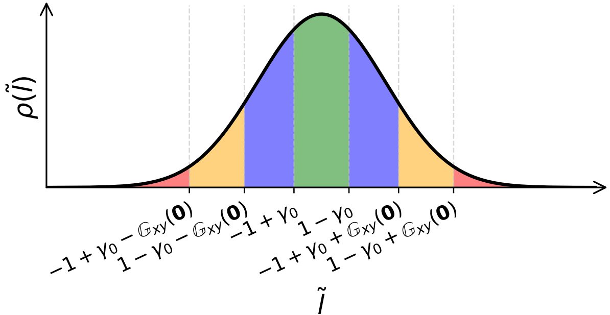
Figure 1.9. Distinct regions of \tilde{l} governing the evolution of an element under oscillatory strain in the deterministic limit l_w = 0 . Elements in the central green region cannot be strained sufficiently to yield and are therefore absorbed. Elements in the blue regions yield on one half-cycle and are mapped into the opposite blue region, allowing them to yield again on the following half-cycle. Elements in the yellow regions yield but are mapped into the central absorbed region. Elements in the red regions have sufficiently large |\tilde{l}| to yield more than once during a single stroke, with repeated yielding reducing |\tilde{l}| until the element enters either a blue or yellow region. The Gaussian profile is shown schematically for clarity and is not intended to represent the instantaneous distribution of \tilde{l} , which will in general be non-Gaussian and vary throughout the oscillation cycle.
