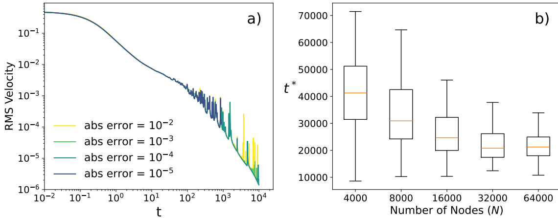
Figure 1.12. Left: Root mean squared velocity against time t for a system strained to \gamma_0 = 1 at t = 0 . We plot the response for four values of absolute error tolerance defined in ???. Right: Convergence of failure time t^* with increasing network size at \gamma_0 = 1 , E = 1.0 , T = 0.0062 .
