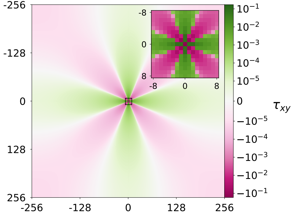
Figure 2. Quadrupolar redistribution of shear stress \tau_{xy} in two dimensions after following a single local normalised point plastic event in a system with \mu = 1 . The system is initialised with \tau_{xy} = 0 everywhere; one central element is then yielded initially unstressed, and the discrete plastic eigenstrain is set to \epsilon_{xy} = -1 at the central grid element and zero elsewhere. The plastic strain, rather than the stress, after which mechanical equilibrium is enforced prescribed at the central element; the resulting equilibrated stress field is calculated using the Fourier-space propagator. The main panel shows the full N_x \times N_y = 512 \times 512 propagator N_x \times N_y = 512 \times 512 field, and the inset shows the central 17 \times 17 region around the propagator.
