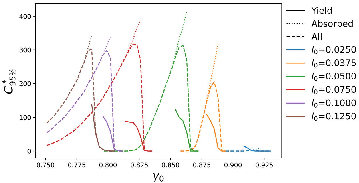
Figure 1.4. Final cycle C^* as a function of the imposed strain amplitude \gamma_0 for various annealing levels l_0 . Smaller values of l_0 correspond to better-annealed samples. We report the 95 th percentile, C^*_{95\%} , defined as the cycle at which the survival distributions in ?? intersect the red threshold line. Results conditioned on yielding and absorption are shown for systems that yield, absorb, or exhibit both behaviours, indicated by solid, dotted, and dashed lines, respectively. For each pair of values for \gamma_0 and l_0 Dashed lines labelled “All” pool all trajectories, the distributions are made up each of at least 10,000 samples which ultimately either yields or reaches an absorbing state. Each parameter combination contains more than 2,500 independent realisations, each run-generated with a different value of the random-number random-number seed; exact ensemble sizes are reported in ??. The curves Outcome-conditioned percentiles are shown in this plot include only those end states for which when more than 1000 such samples 2,500 realisations reach the corresponding outcome end state.
