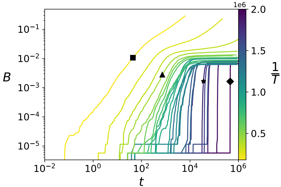
Figure 1.11. Fraction of broken bonds B as a function of time t following the imposition of a step strain of amplitude \gamma_0 = 0.01 , with bond breakage energy E = 5.025 \times 10^{-5} . Here, B := N_b/N denotes the fraction of broken bonds relative to the total initial number of bonds N_{\text{tot}} = 64,000 . The colour scale indicates the temperature T associated with each curve. The symbols show the location of snapshots in ??.
