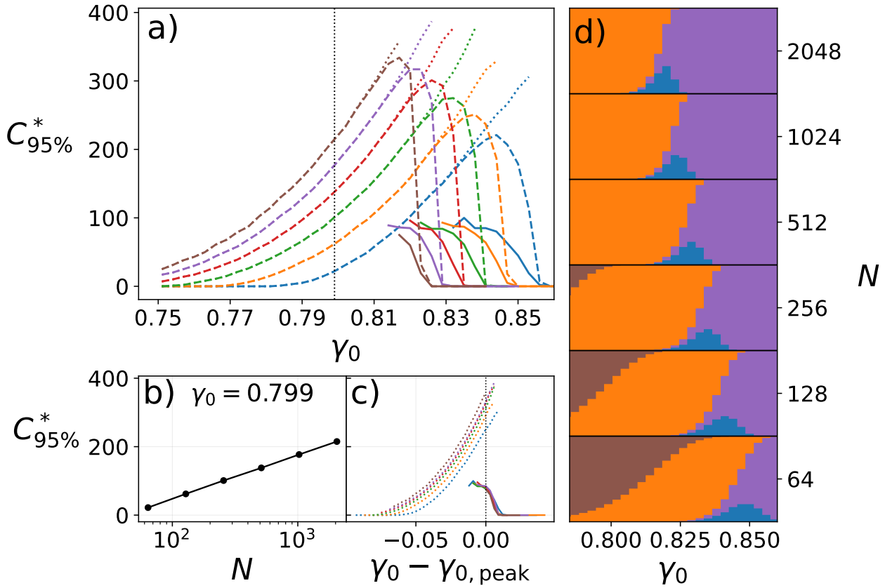
Figure 1.6. Effect of system size N at fixed parameters l_0 = 0.075 and l_w = 0.02 .
