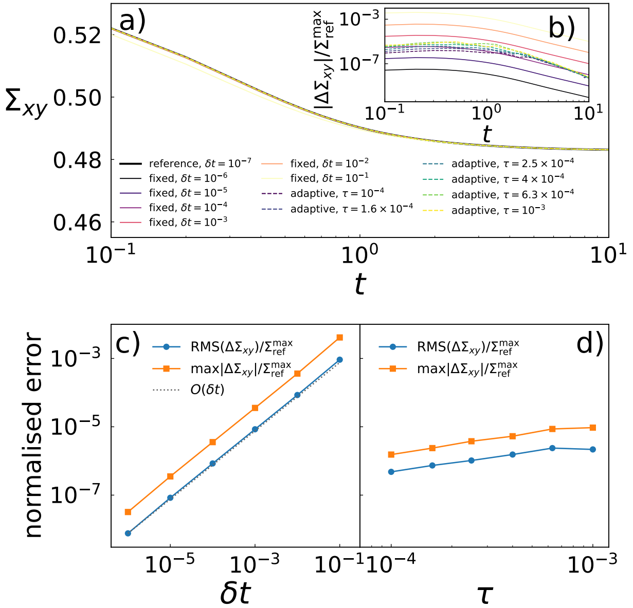
Figure 4. Numerical convergence of the overdamped network dynamics over 0 \leq t \leq 10 . (a) Bulk shear stress \Sigma_{xy}(t) for all fixed Euler and adaptive Euler-Heun trajectories, including the fixed reference trajectory ( \delta t_{\text{ref}} = 10^{-7} ). (b), inset Corresponding pointwise normalised absolute errors |\Delta\Sigma_{xy}(t)|/\Sigma_{\text{ref}}^{\text{max}} for every non-reference trajectory. (c) Normalised RMS and maximum errors for fixed Euler trajectories, demonstrating first-order convergence with \delta t . (d) The same normalised errors as functions of the absolute tolerance \tau over the rounded logarithmic grid from 10^{-4} to 10^{-3} .
