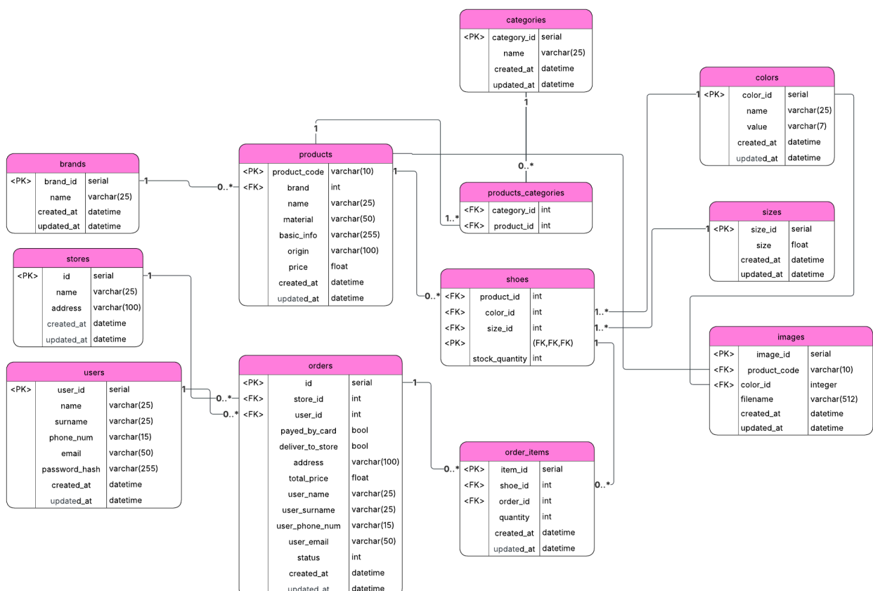
Figure 1: PHYSICAL DATA MODEL OF OUR RELATION DATABASE
