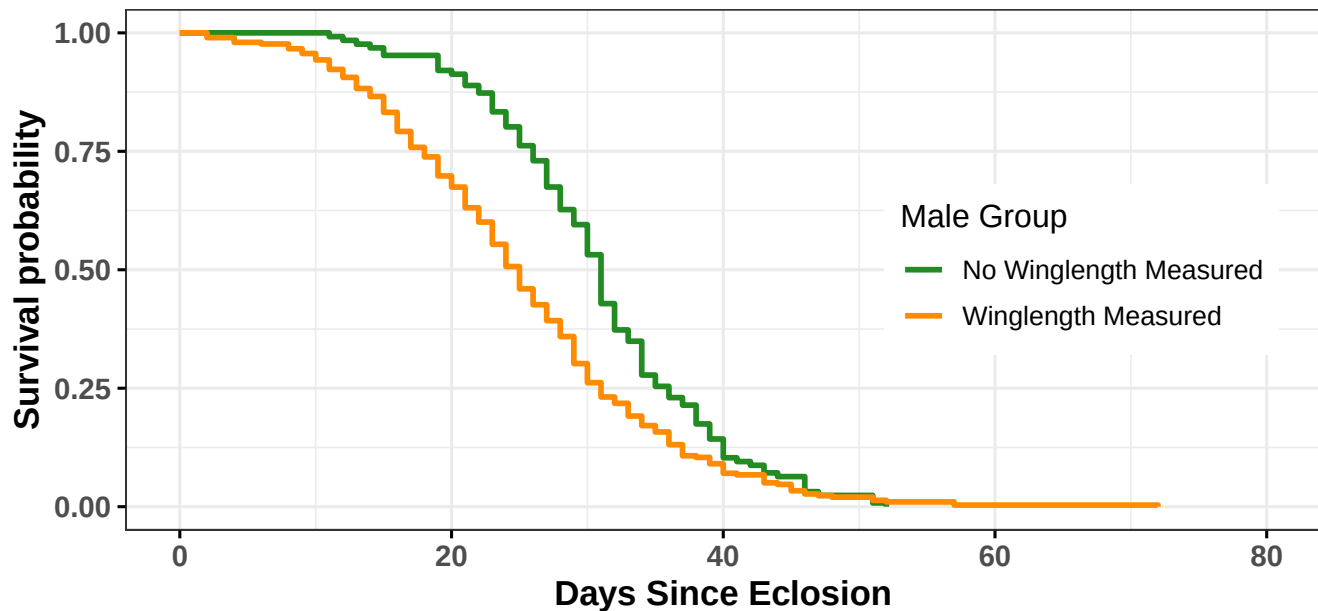
Figure 3: Survival curve comparing males with wing-length measurements to those where wing-length was not capable of being measured. The males missing wing-length data had greater survival than those with wing length data ( p = 7.42 \times 10^{-5} ).
