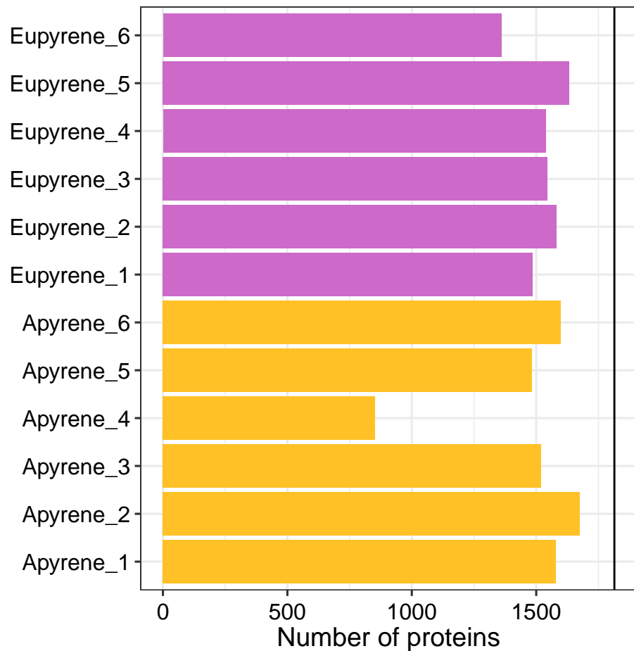
Protein counts
