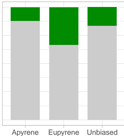
Signal peptide
