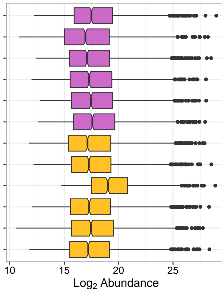
Protein abundance
