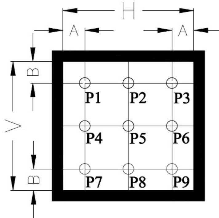
A : H/6 ; B : V/6 ; H,V : Active Area(AA) size Measurement instrument: BM-7; Light spot size=5mm, 350mm distance from the LCD surface to detector lens.
