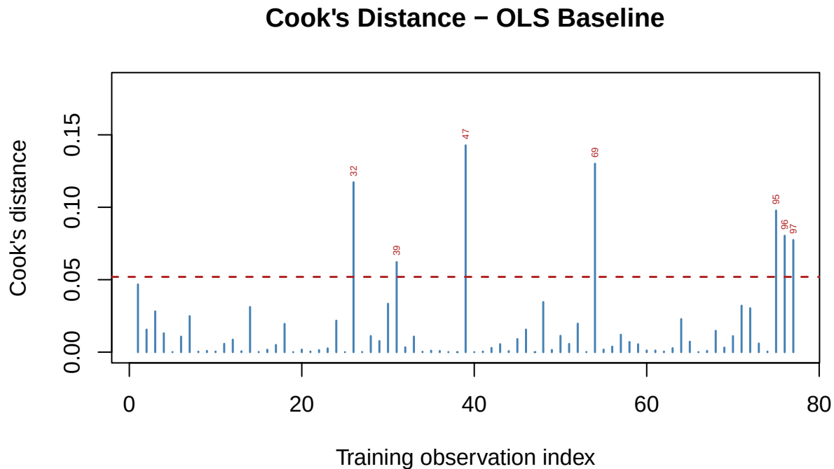
Figure 2: Cook's distance for the OLS fit. Bars above the dashed 4/n threshold are flagged as influential; each flagged bar is labelled with its row number in the original prostate.csv, not its training position.
