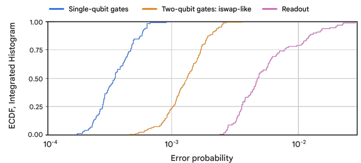
Willow Chip 2: RCS
