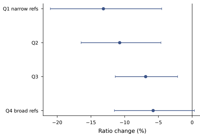
Paper reference breadth, with no subgroup selection
