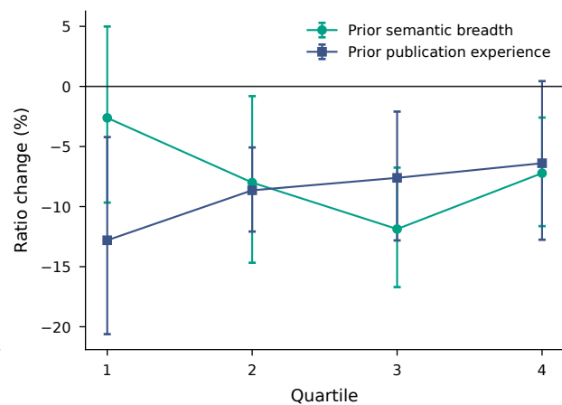
Author history
