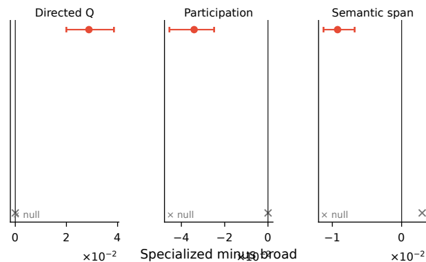
c Three network summaries
