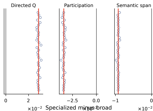
d Direction after omitting each source domain
