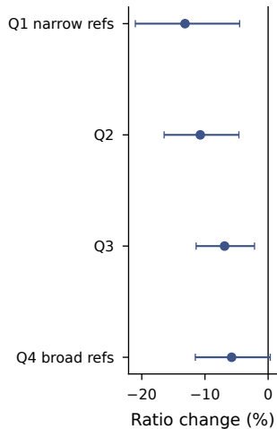
c Reference breadth
