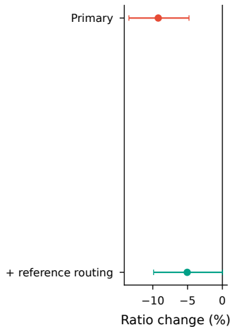
b Reference-inclusive model
