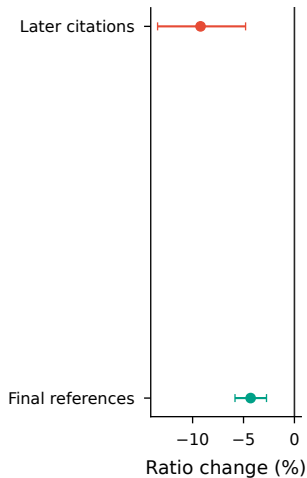
a Reference routing
