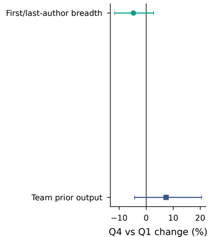
d Author history
