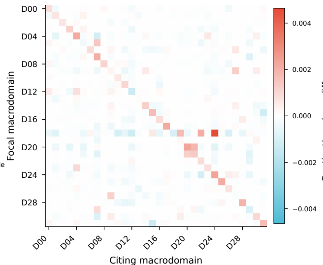
b All 1,024 source-destination cells
