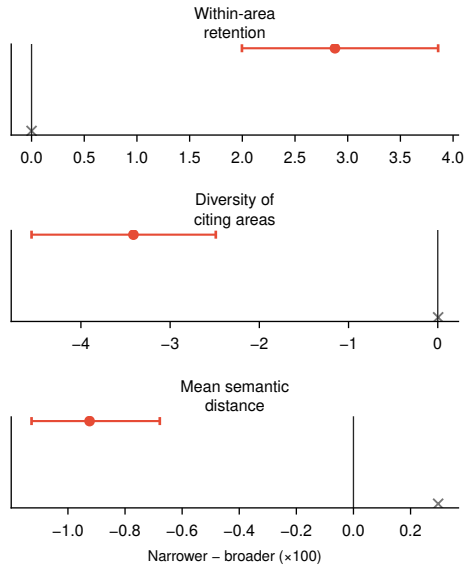
Three views of citation concentration
