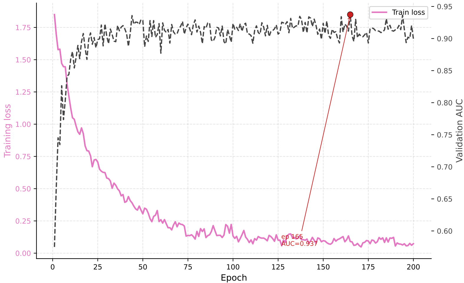
CasGNet w/o GRN
