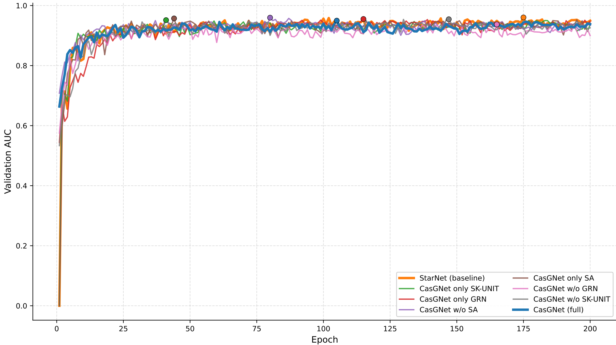
Ablation — Validation AUC (all variants)
