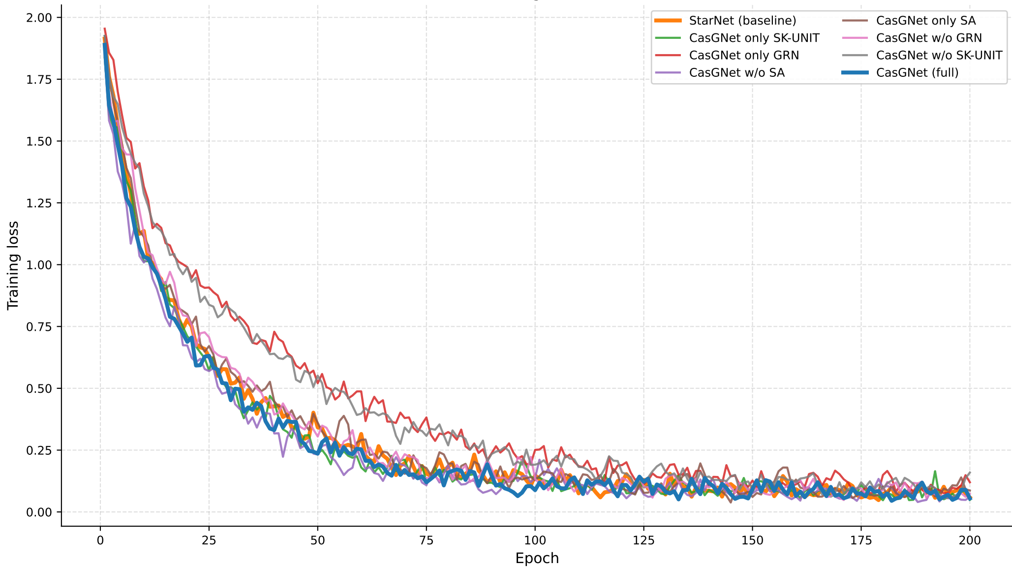
Ablation — Training Loss (all variants)
