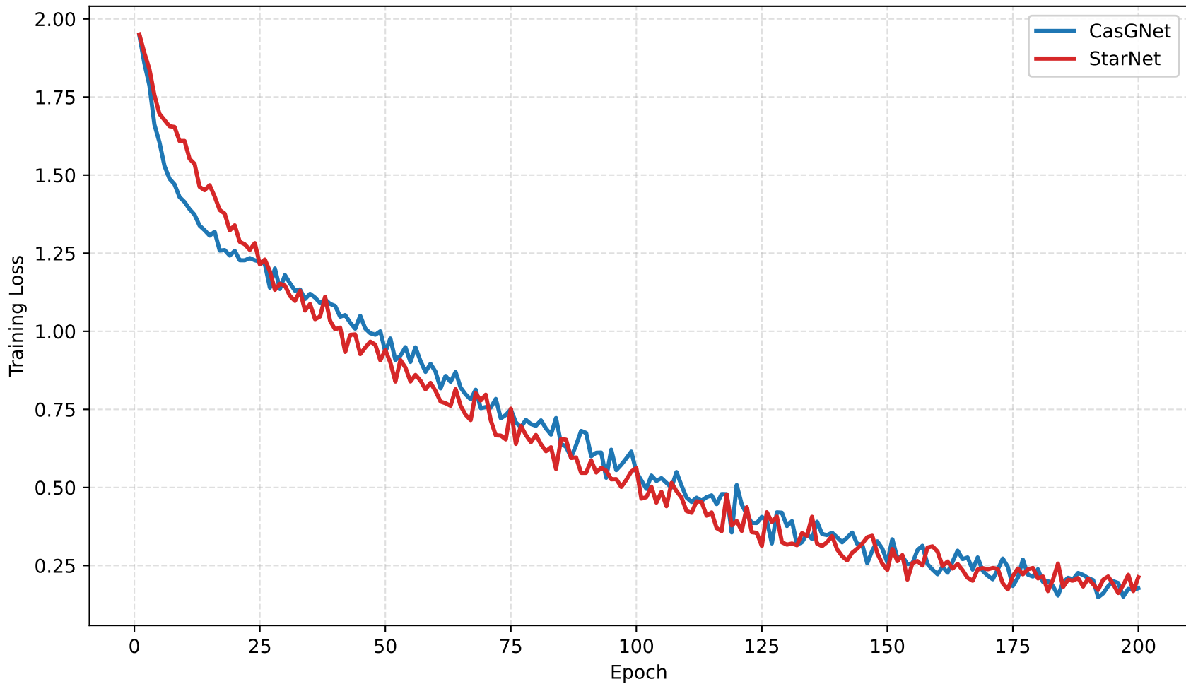
Training Loss: CasGNet vs StarNet
