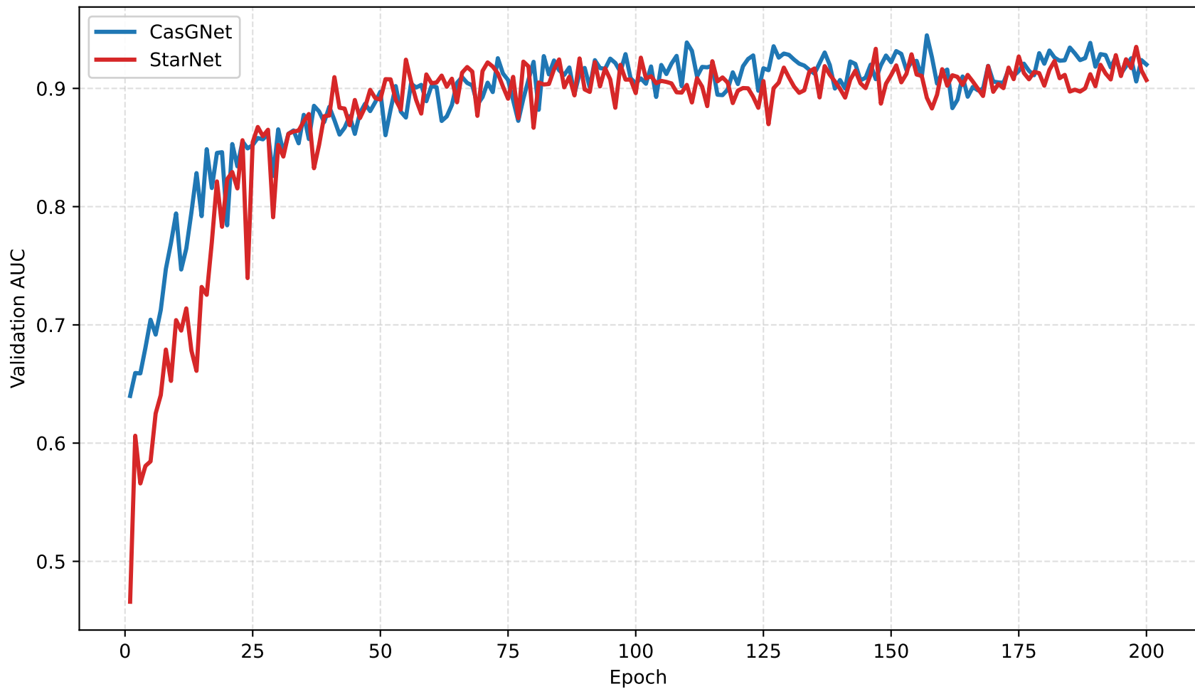
Validation AUC: CasGNet vs StarNet
