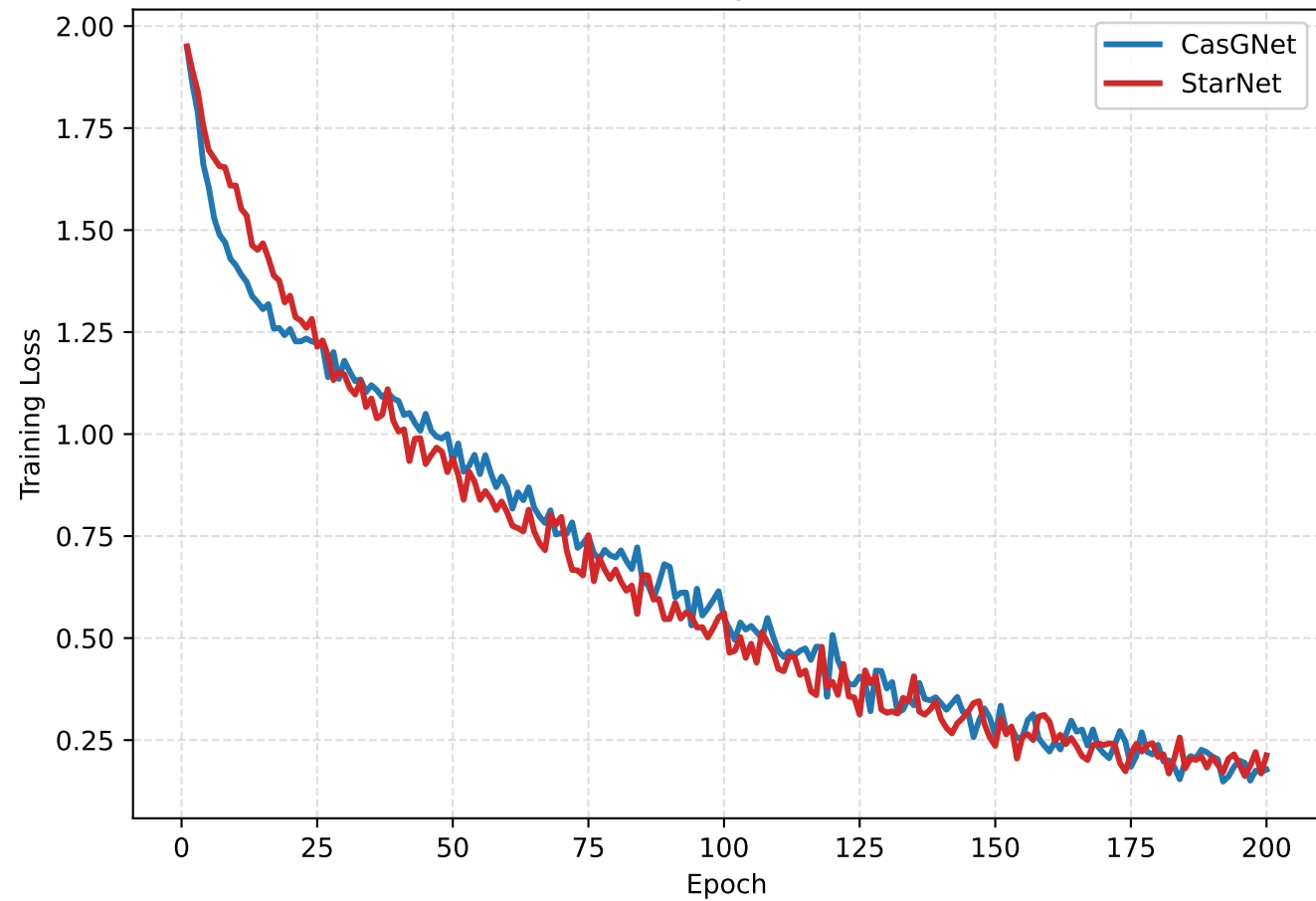
Training Loss
