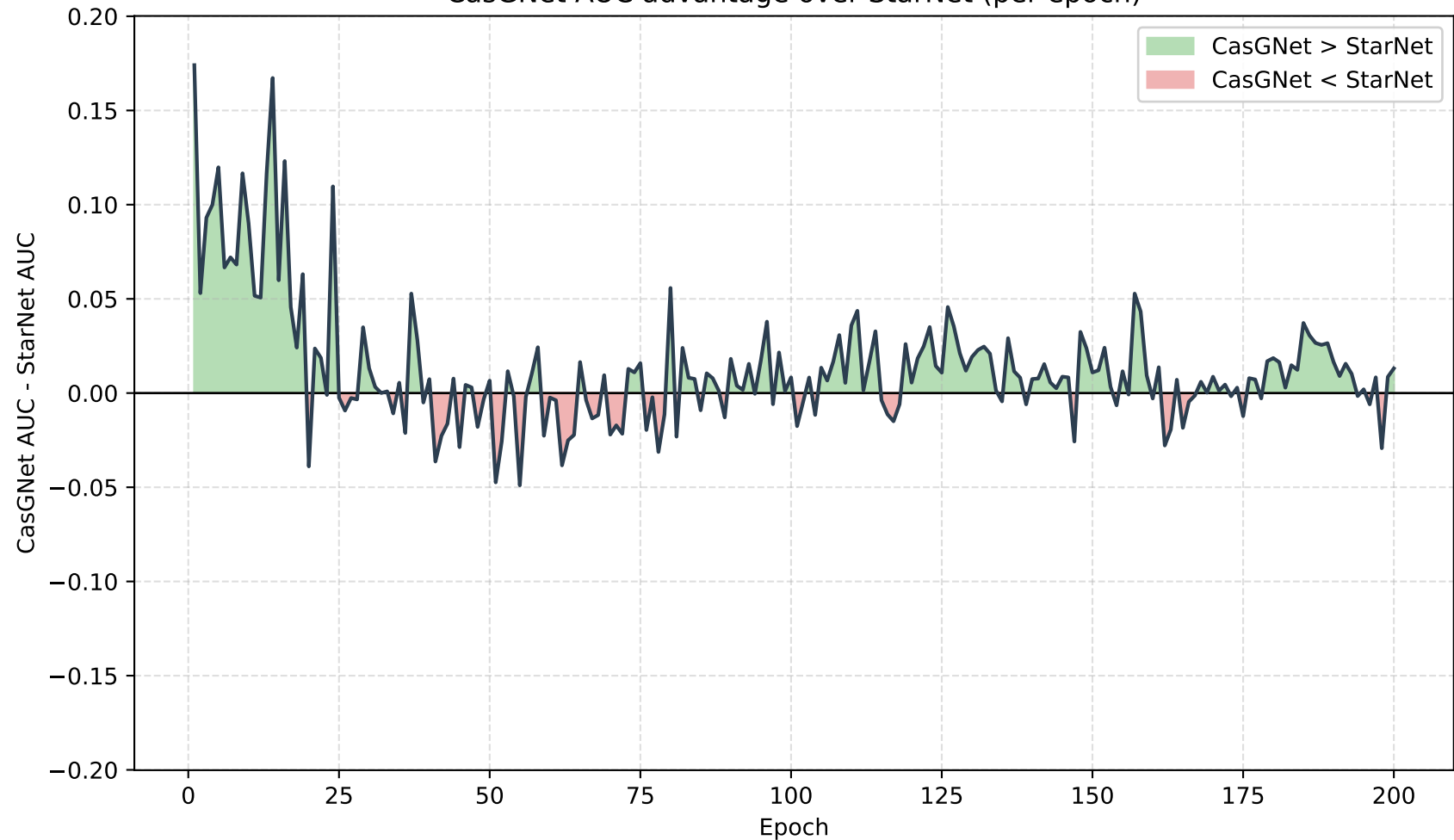
CasGNet AUC advantage over StarNet (per epoch)
