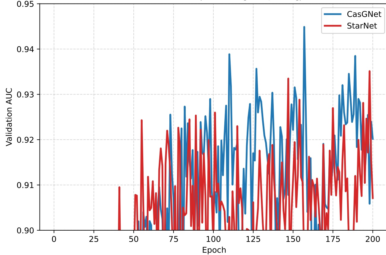
Validation AUC (zoomed [0.90, 0.95])
