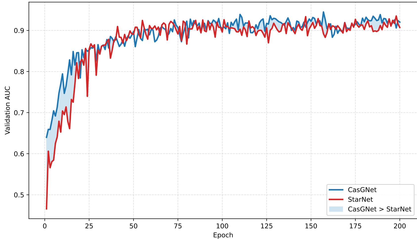
Validation AUC: CasGNet vs StarNet (gap shaded)
