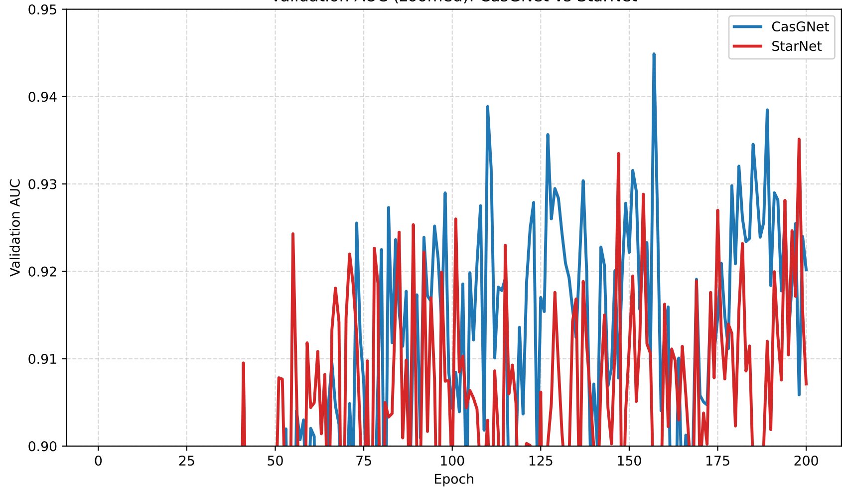
Validation AUC (zoomed): CasGNet vs StarNet
