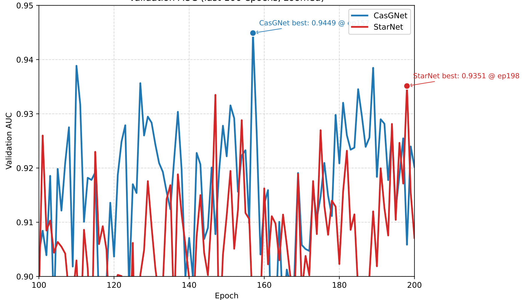
Validation AUC (last 100 epochs, zoomed)
