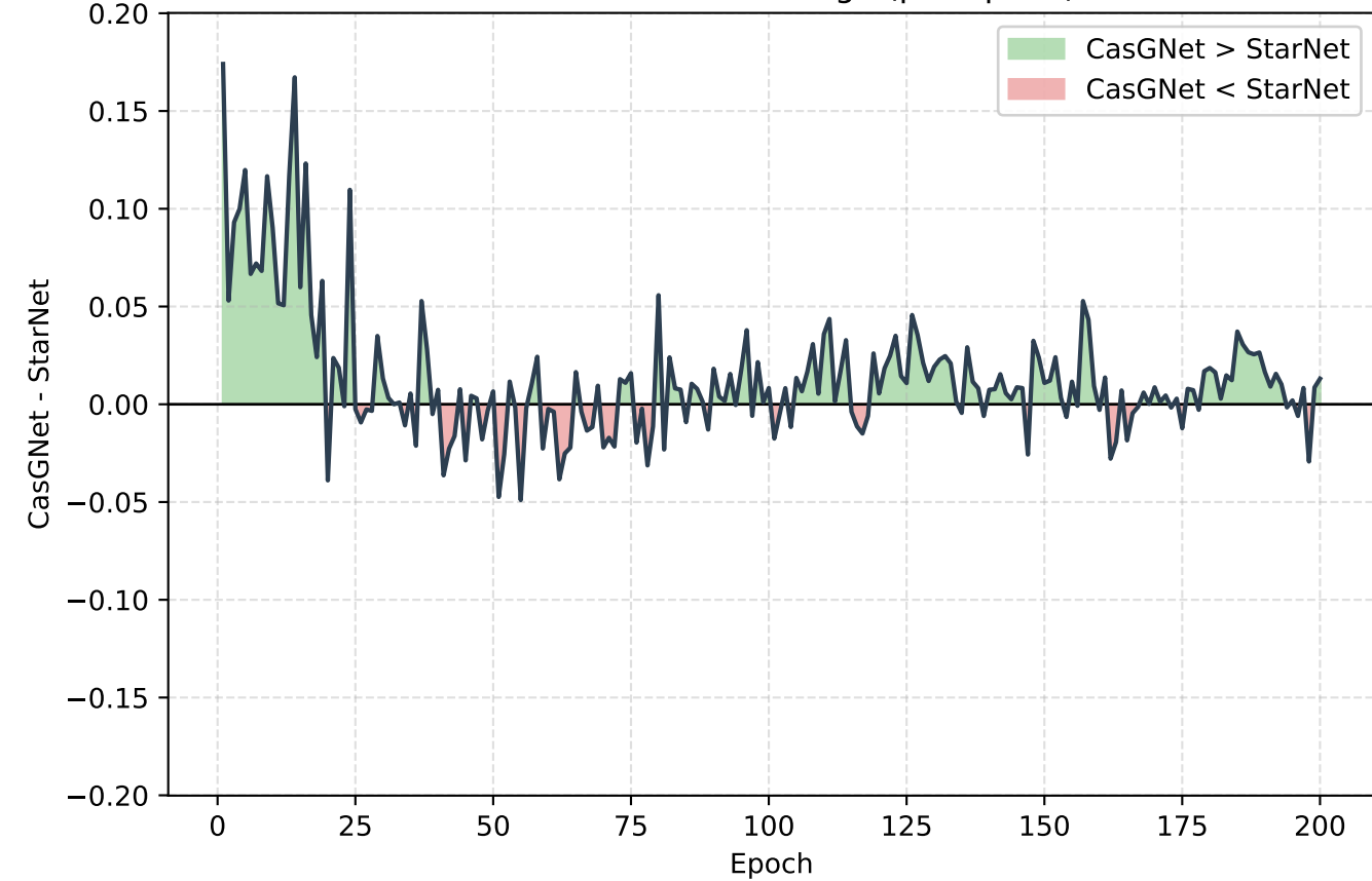
CasGNet AUC advantage (per epoch)
