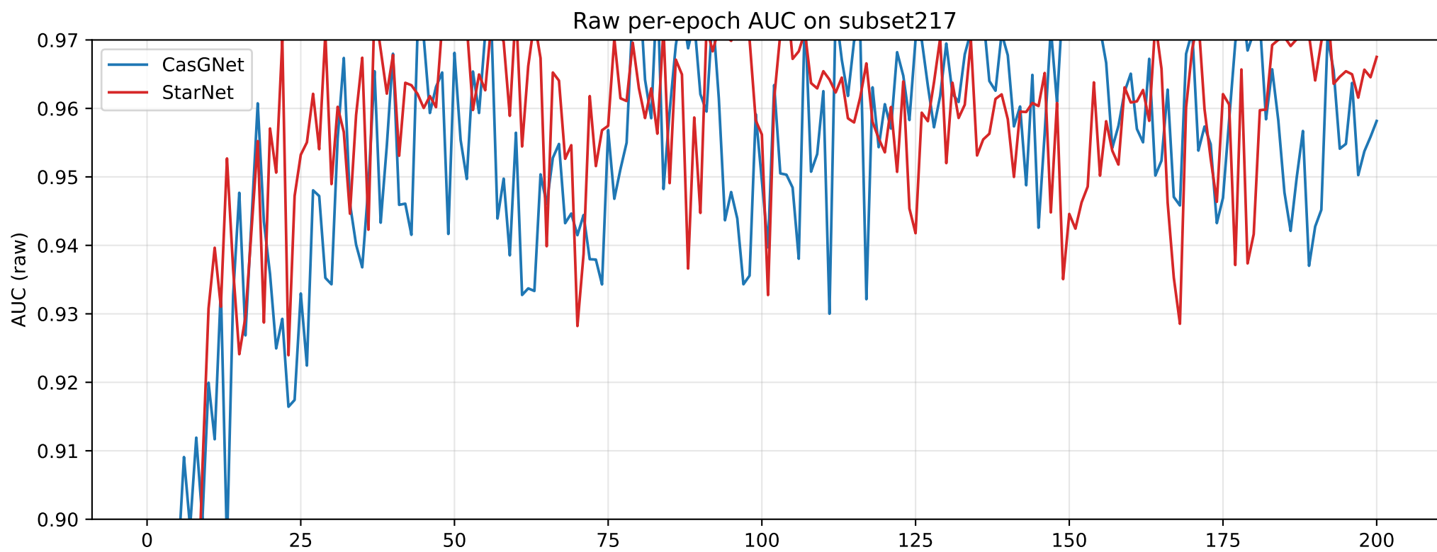
subset217 per-epoch AUC: CasGNet vs StarNet (retrain + per-epoch eval)
