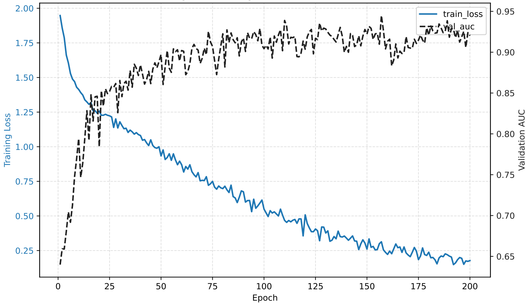
casgnet - Training Loss & Validation AUC
