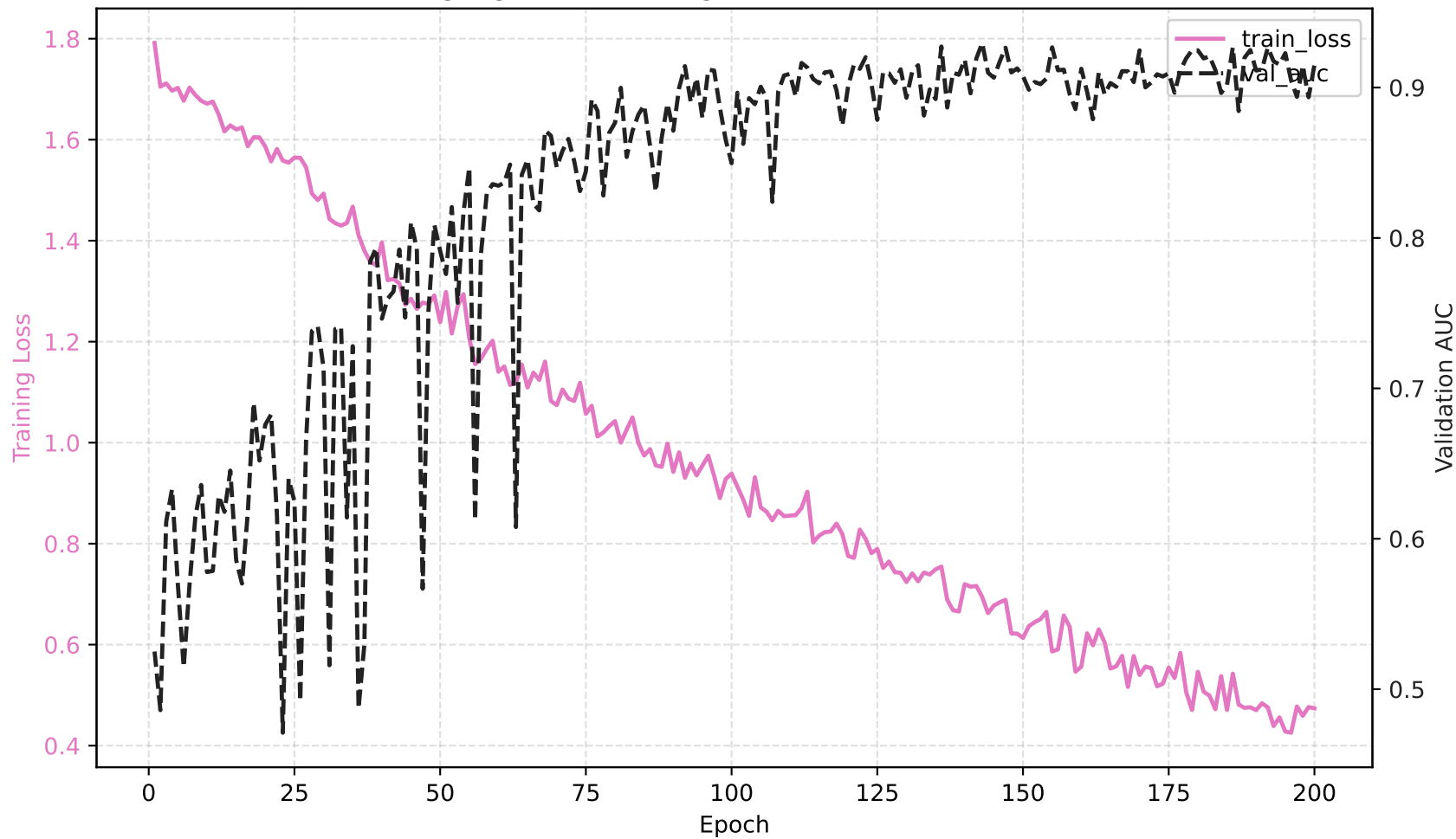
googlenet - Training Loss & Validation AUC
