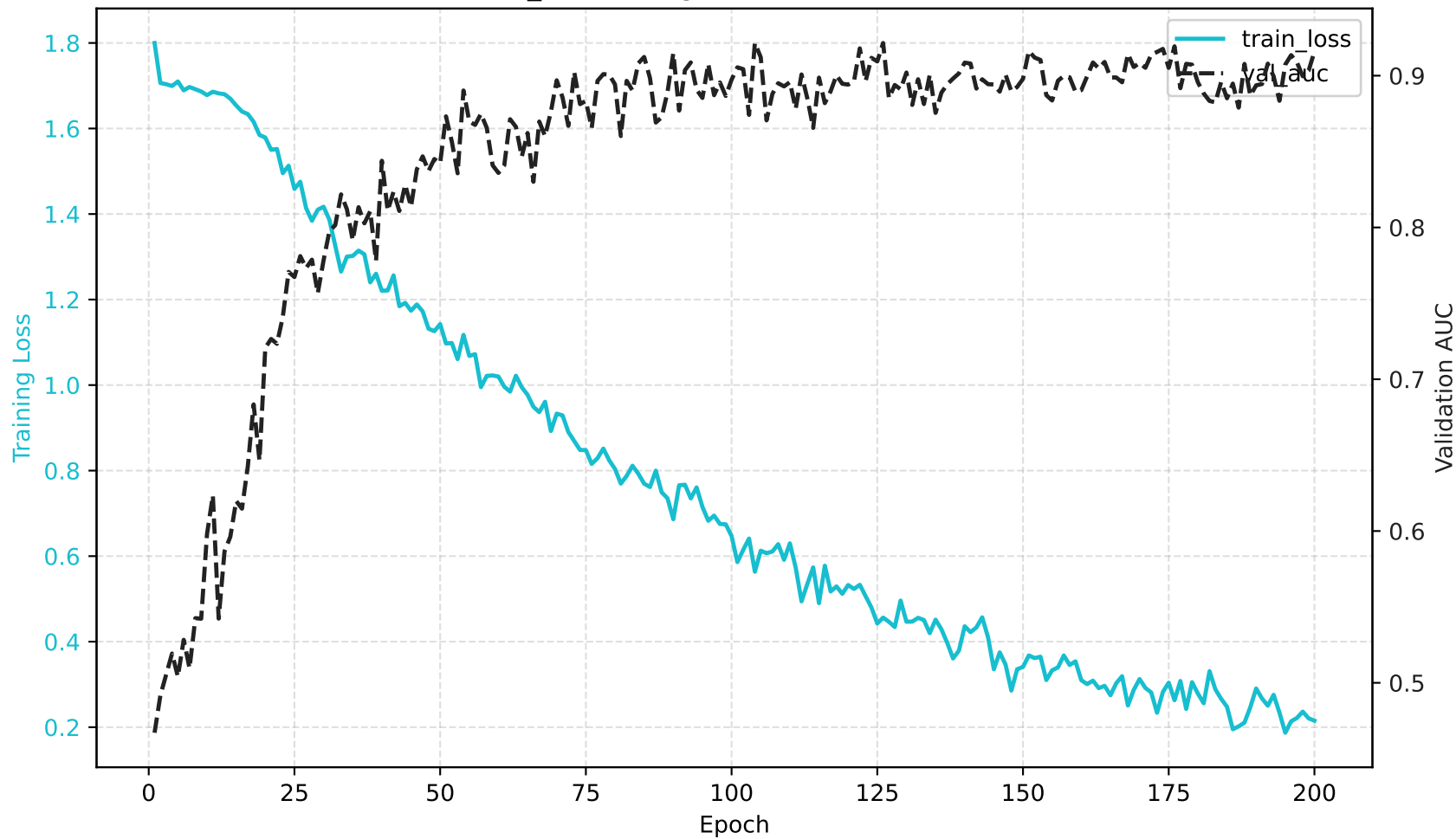
Isnet_b - Training Loss & Validation AUC
