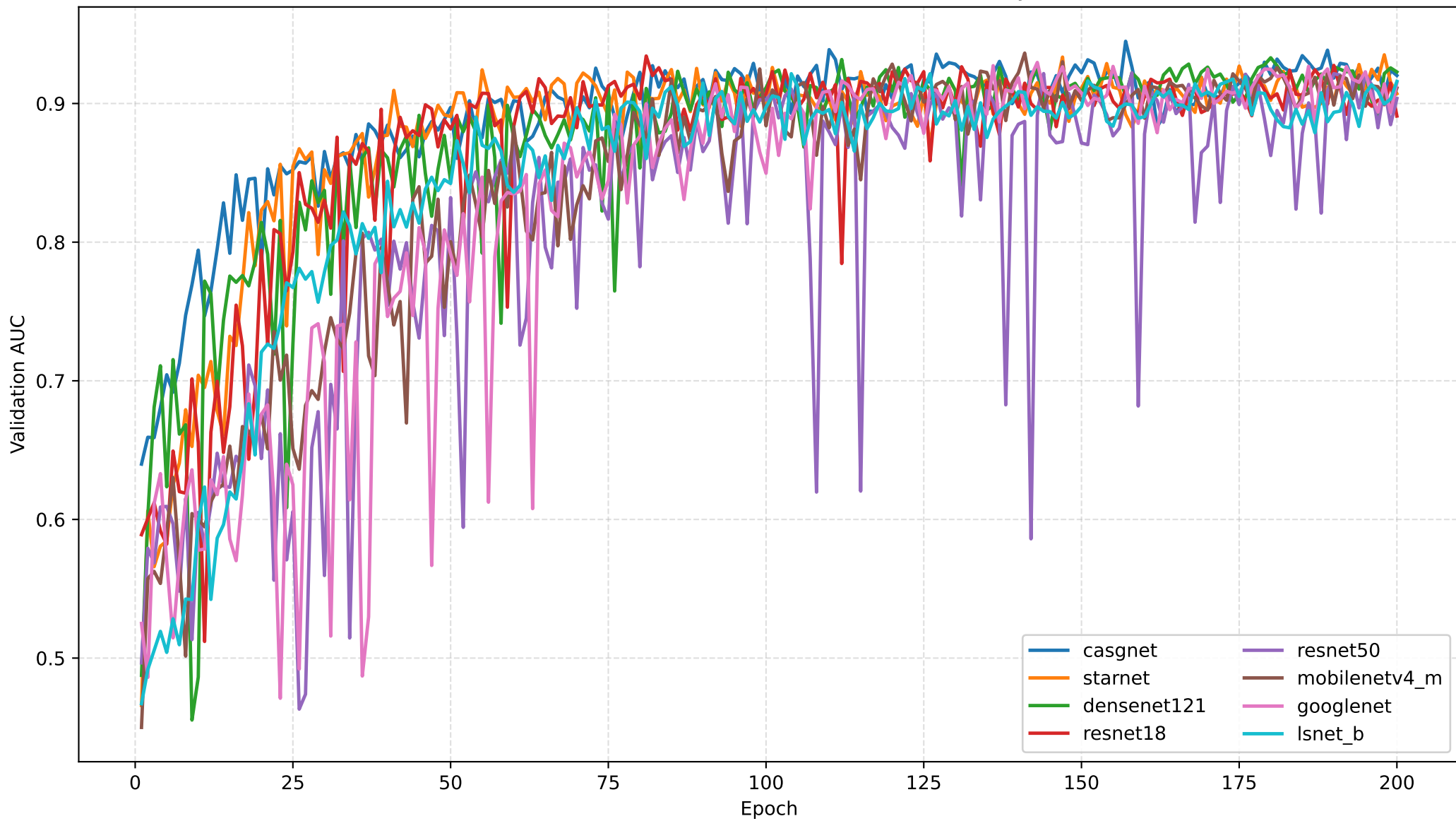
Validation AUC Curves (8 Main Models, CE-only)
