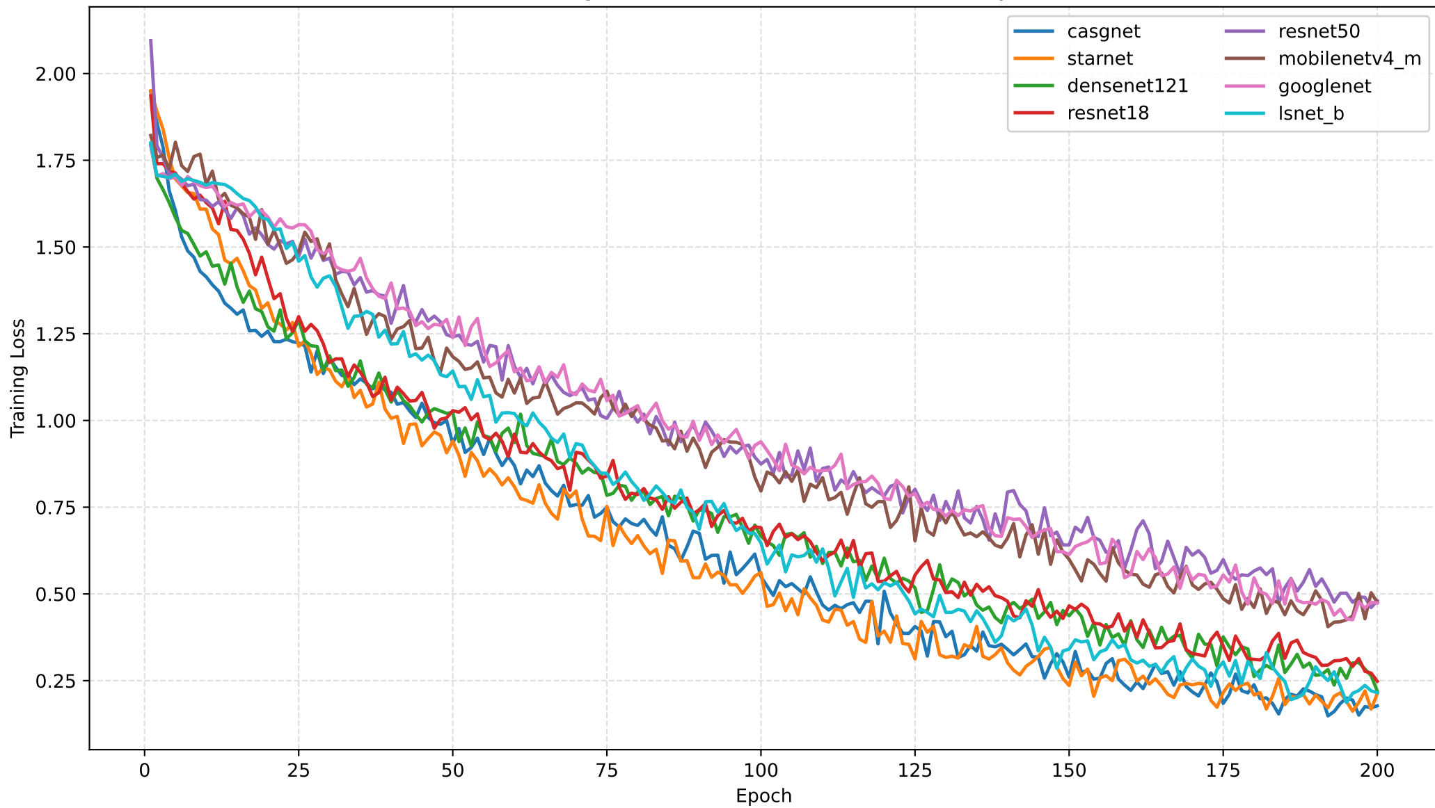
Training Loss Curves (8 Main Models, CE-only)
