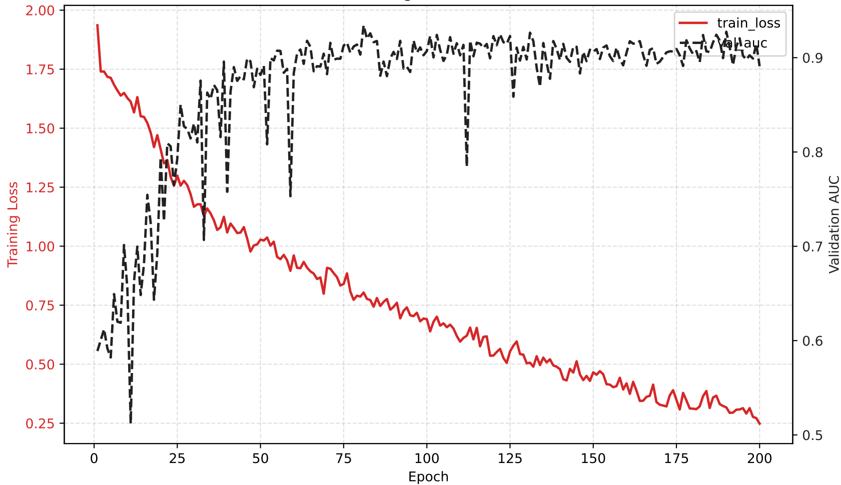
resnet18 - Training Loss & Validation AUC
