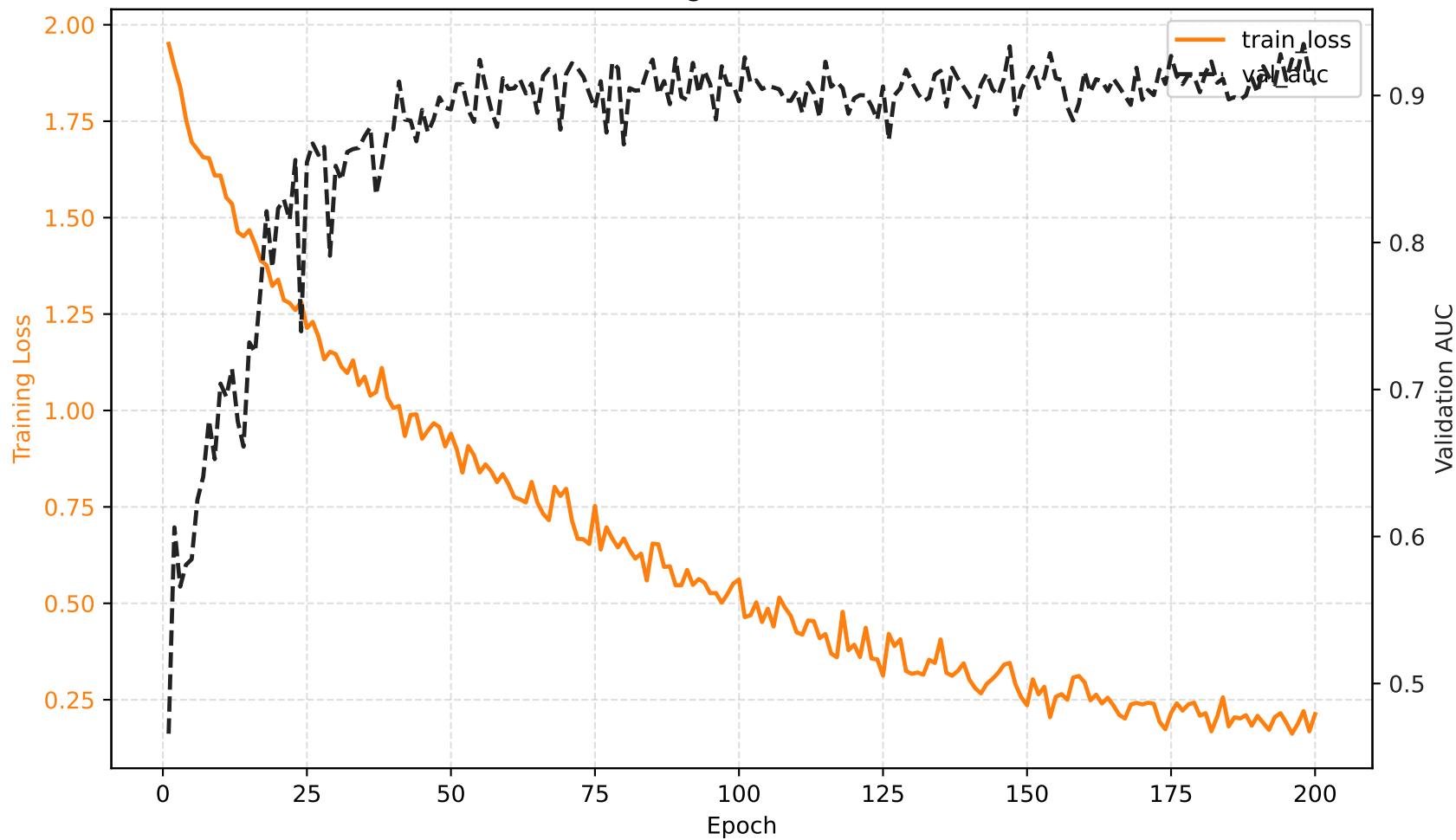
starnet - Training Loss & Validation AUC
