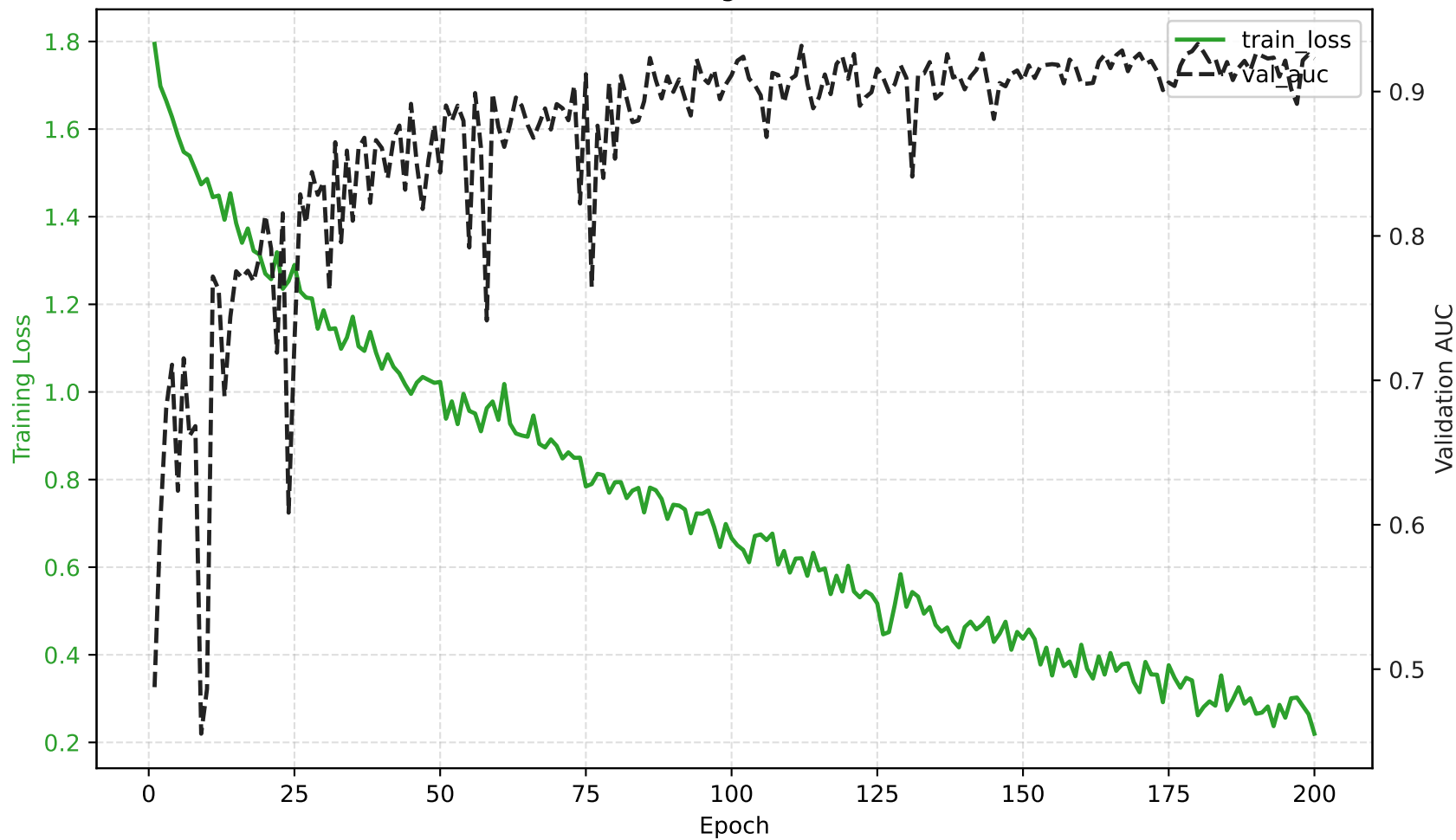
densenet121 - Training Loss & Validation AUC
