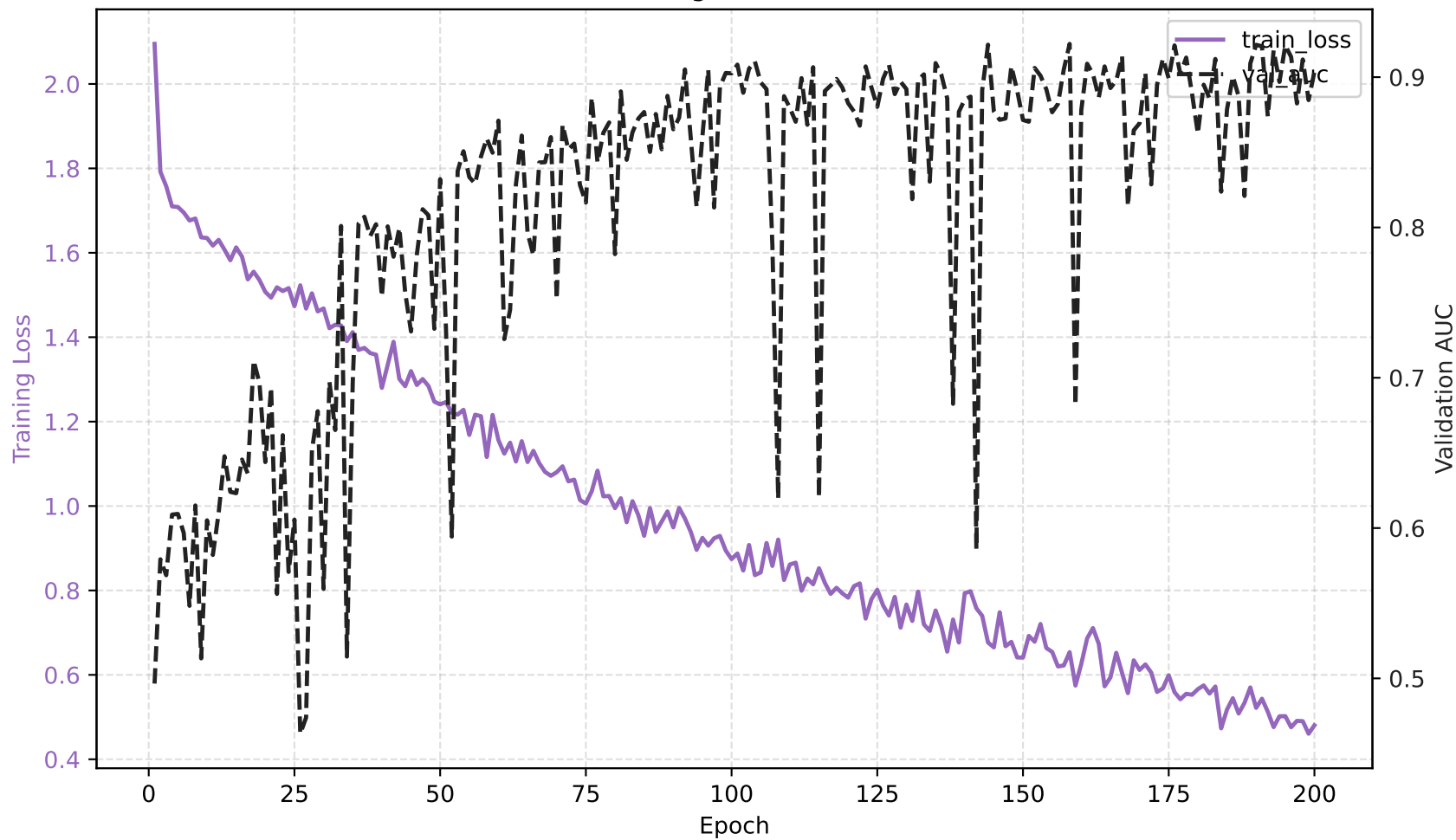
resnet50 - Training Loss & Validation AUC
