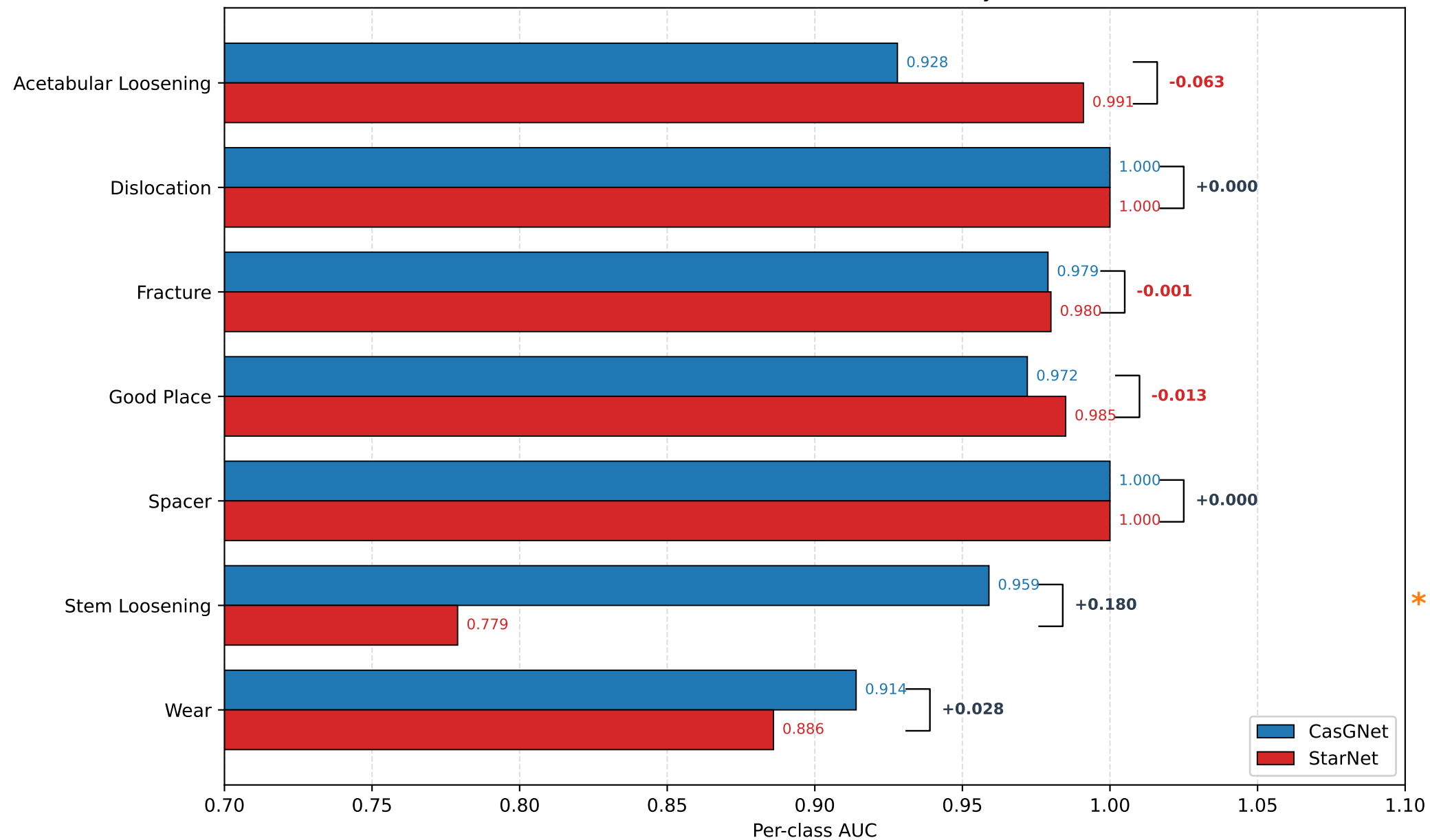
Per-class AUC: CasGNet vs StarNet (Table1, subset217, n=230)
