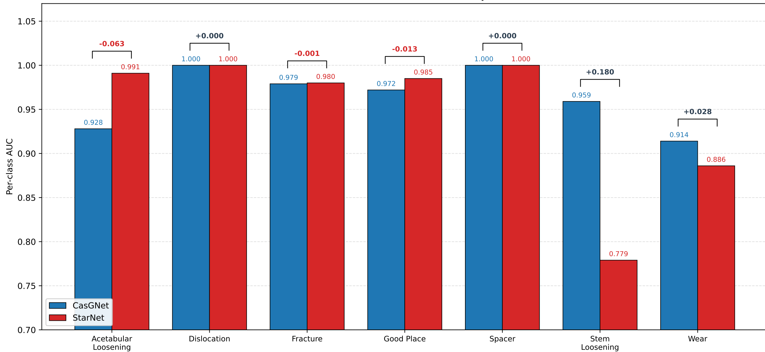
Per-class AUC: CasGNet vs StarNet (Table1, subset217, n=230)
