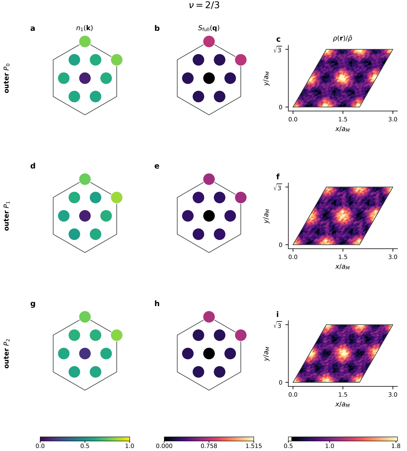
Figure 8: \nu = 2/3 outer-sector observables from equilibrated training samples. Rows are P_0, P_1, P_2 and columns use the same definitions and global color limits as Fig. 7. All panels use 4,128 configurations and 16 jointly batched auxiliary replacements per configuration. The three sectors are shown separately because both their band populations and two-body structure factors differ beyond a simple identical-map interpretation.
