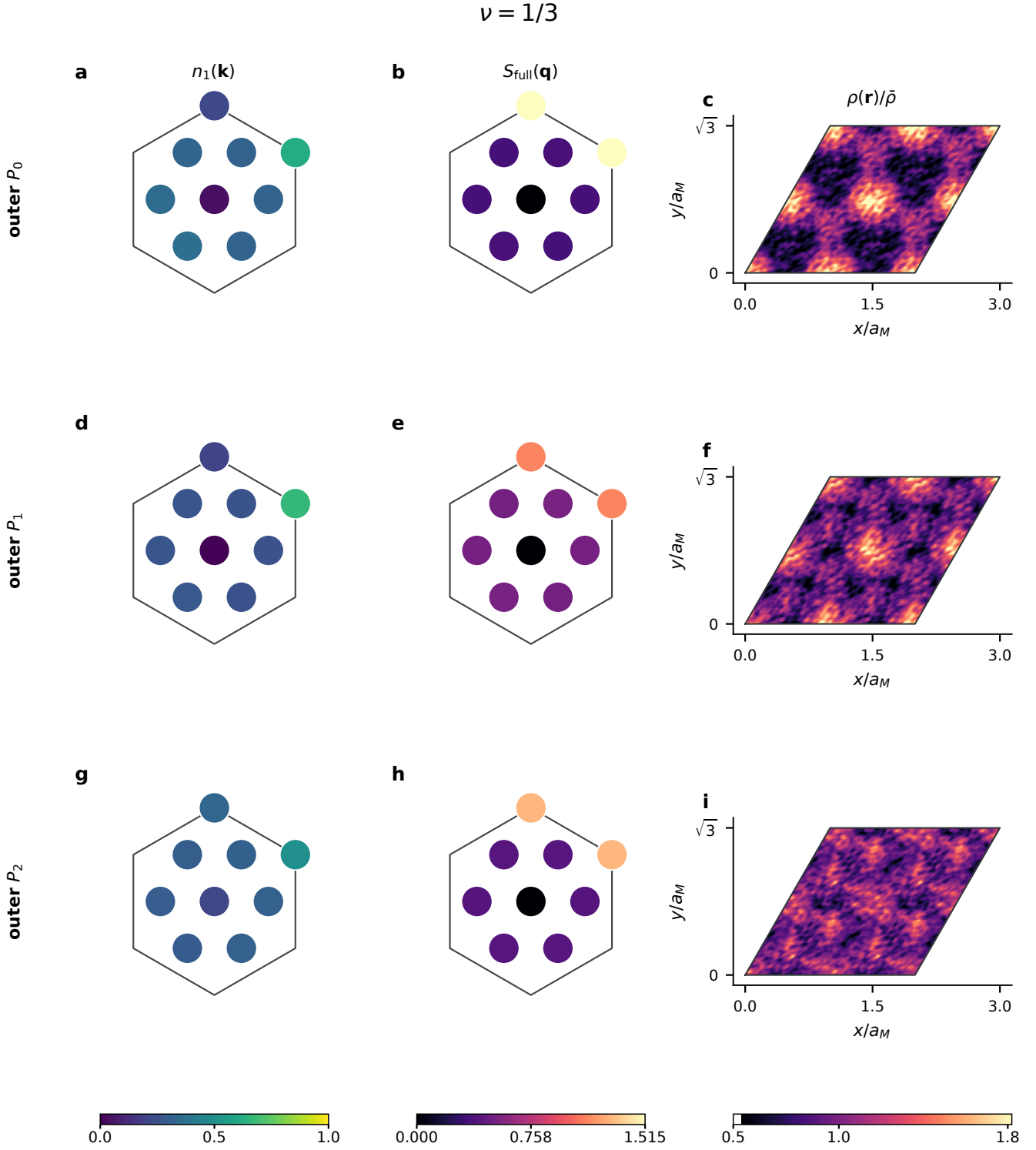
Figure 7: \nu = 1/3 outer-sector observables from equilibrated training samples. Rows are complete-wavefunction projectors P_0, P_1, P_2 . Columns show bare-band-1 momentum occupation from the complete-ratio 1-RDM, the full static structure factor with ED normalization on the complete hexagonal BZ, and folded charge density over a two-by-two moiré-cell parallelogram. Shared color limits expose the strong P_1 band-mixing and structure-factor difference without rescaling individual sectors.
