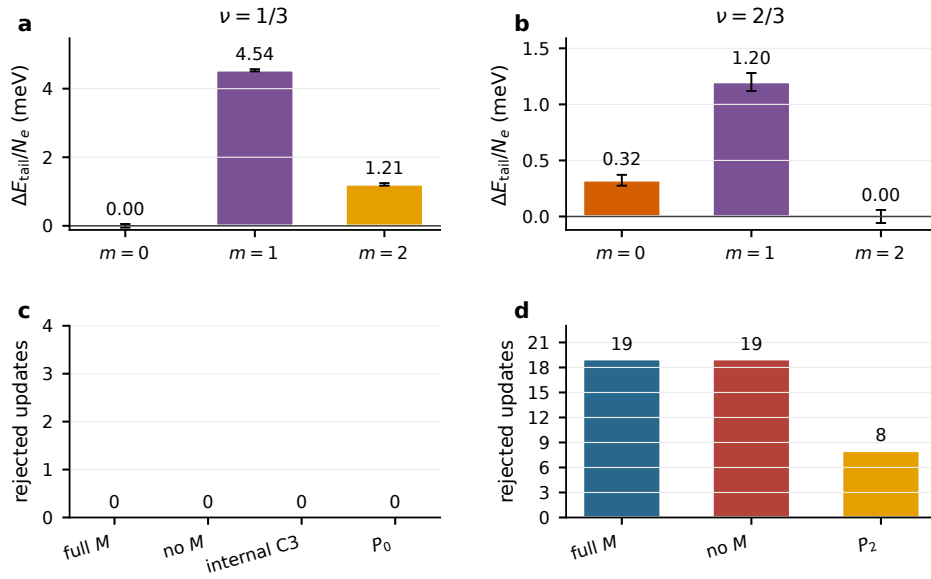
Figure 7: Outer- C_3 sector splitting and optimizer stability. (a,b) Final-ten energy offsets of the externally projected P_m states, measured from the lowest sector at each filling. Error bars are RMS fluctuations of the correlated training tail, not independent standard errors. At \nu = 1/3 , m = 0 is selected, while m = 1, 2 lie 4.537 and 1.209 meV per particle higher. At \nu = 2/3 , m = 2 is selected, with m = 0, 1 higher by 0.323 and 1.199 meV per particle. The smaller spread at \nu = 2/3 is compatible with, but does not establish, the expected quasi-degenerate FCI manifold. (c,d) Cumulative rejected parameter updates for the methods retained in Fig. 6; rejection concerns an optimizer step, not a Monte Carlo configuration.
