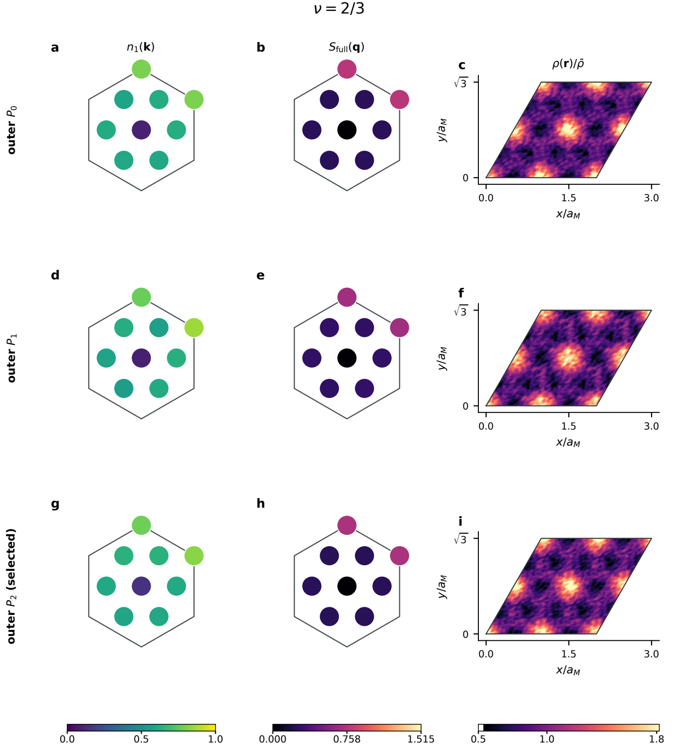
Figure 9: \nu = 2/3 outer-sector observables from equilibrated training samples. Rows are P_0, P_1, P_2 and columns use the same definitions and global color limits as Fig. 8. All panels use 4,128 configurations and 16 jointly batched auxiliary replacements per configuration. The three sectors are shown separately because both their band populations and two-body structure factors differ beyond a simple identical-map interpretation.
