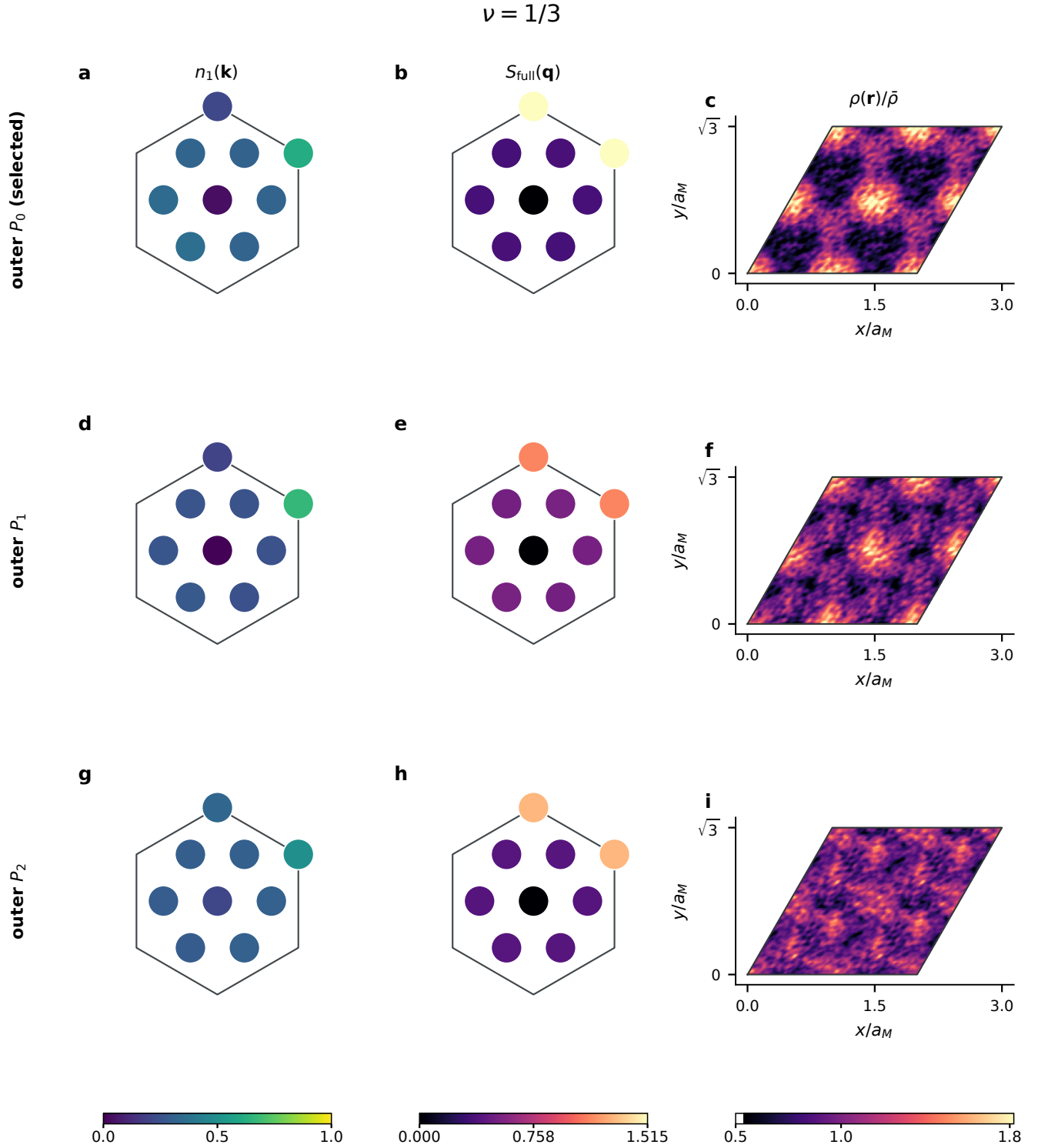
Figure 8: \nu = 1/3 outer-sector observables from equilibrated training samples. Rows are complete-wavefunction projectors P_0, P_1, P_2 ; the first row, P_0 , is the selected out- C_3 state because it has the lowest final-ten training energy. Columns show bare-band-1 momentum occupation from the complete-ratio 1-RDM, the full static structure factor with ED normalization on the complete hexagonal BZ, and folded charge density over a two-by-two moiré-cell parallelogram. Shared color limits expose the strong P_1 band-mixing and structure-factor difference without rescaling individual sectors.
