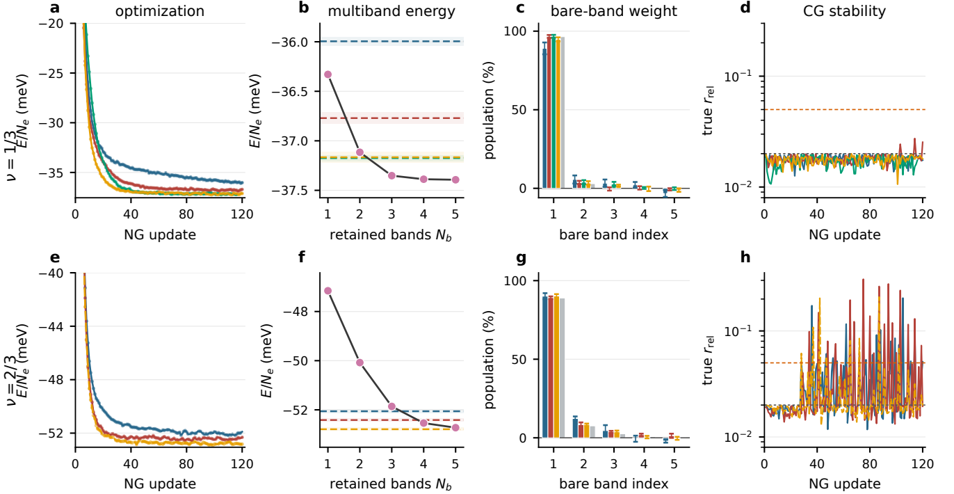
Figure 6: Controlled neural-Bloch optimization, multiband energy, band mixing and CG stability. Top row: \nu = 1/3 ; bottom row: \nu = 2/3 . Blue, red and green denote full M , no M and internal C3-QNS; orange denotes the lowest final-ten outer sector, P_0 at \nu = 1/3 and P_2 at \nu = 2/3 . Internal C3 exists only in the upper row and stops at update 116. (a,e) Persistent-walker training energies. (b,f) One- through five-band ED energies and final-ten training means; shaded widths are the corresponding RMS, not independent error bars. (c,g) Bare-band populations from the complete-wavefunction-ratio 1-RDM, including the lowest-training outer sector and five-band ED in gray. (d,h) Explicit true CG residuals; horizontal lines mark the 0.02 early-stop and 0.05 cap-acceptance thresholds. Rejected-update counts are summarized separately in the text.
