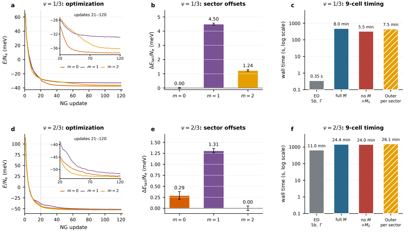
Figure 7: Outer- C_3 optimization, sector splitting and efficiency. (a,d) All three sector-energy traces at \nu = 1/3 and 2/3 , respectively, with the complete 120-update history and insets resolving updates 21–120. The dotted line marks the end of shared mixture sampling at update 20; projected parameters update independently throughout both fillings’ runs. (b,e) Final-ten energy offsets of the externally projected P_m states, measured from the lowest sector at each filling. Error bars are RMS fluctuations of the correlated training tail, not independent standard errors. At \nu = 1/3 , m = 0 is selected, while m = 1, 2 lie 4.499 and 1.236 meV per particle higher. At \nu = 2/3 , m = 2 is selected, with m = 0, 1 higher by 0.292 and 1.310 meV per particle. Incomplete convergence, particularly in P_1 , prevents interpreting these splittings as a converged FCI manifold. (c,f) Separate nine-cell timing comparisons at \nu = 1/3 and 2/3 on a common logarithmic seconds axis. Five-band ED in \Gamma takes 0.349 s (median of five fresh processes) and 11.0 min, respectively, for four eigenpairs. Full M and no M+M_S show their individual 120-update job times, excluding validation, export and observables. For the hatched outer bars, 7.5 and 26.1 min/sector at \nu = 1/3 and 2/3 are the respective total wall times divided by three candidate states. This amortized measure is not a standalone state’s runtime. Different scopes and total resource costs are specified in Table 9; no Berry or 27-cell spectrum time enters this comparison.
