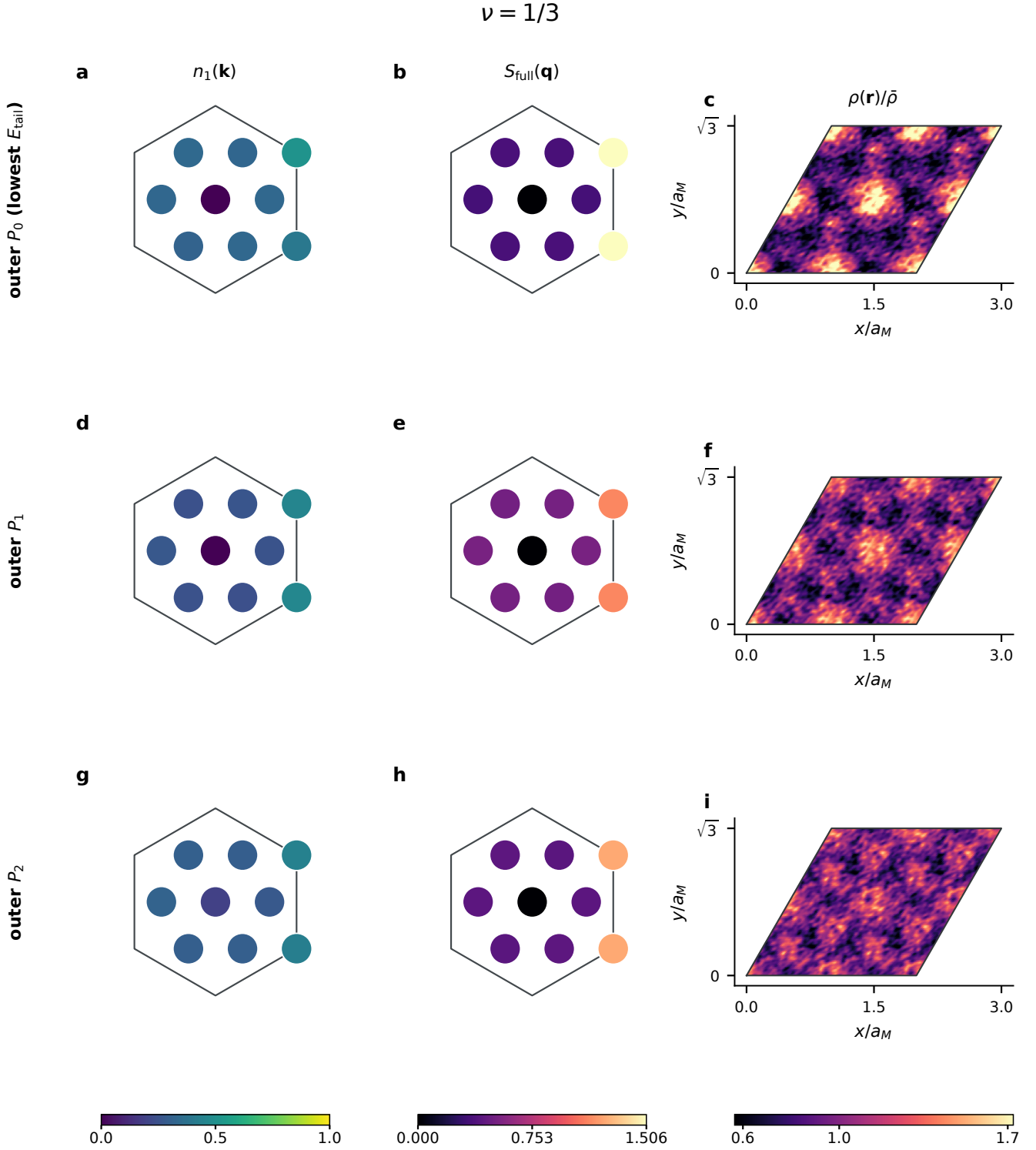
Figure 9: \nu = 1/3 outer-sector observables from final training samples. Rows are complete-wavefunction projectors P_0, P_1, P_2 ; the first row, P_0 , is explicitly marked as the selected outer- C_3 state because it has the lowest final-ten training energy. Columns show bare-band-1 momentum occupation from the complete-ratio 1-RDM, the full static structure factor with ED normalization on the complete hexagonal BZ, and folded charge density over a two-by-two moiré-cell parallelogram. Shared color limits expose the strong P_1 band-mixing and structure-factor difference without rescaling individual sectors.
