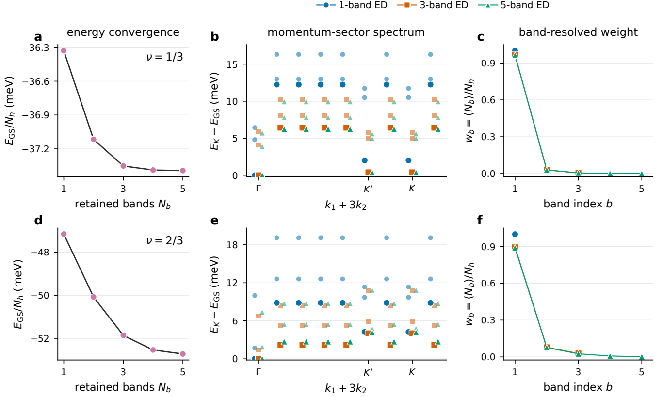
Figure 2: Multiband ED on the 3 \times 3 cluster. Top row: \nu = 1/3 ; bottom row: \nu = 2/3 . (a,d) Ground-state energy per hole versus retained bands; filling labels are placed in the upper-right blank region. (b,e) The lowest three levels in every momentum sector for one-, three- and five-band ED, plotted as E - E_{GS} in meV. Larger opaque markers denote sector ground states; the next two levels are smaller and semitransparent. (c,f) Normalized band-resolved ground-state weights. Charge- U(1) , spin- U(1) and translations are exact; C_3/C_6 equivalence accelerates the largest five-band sectors.
