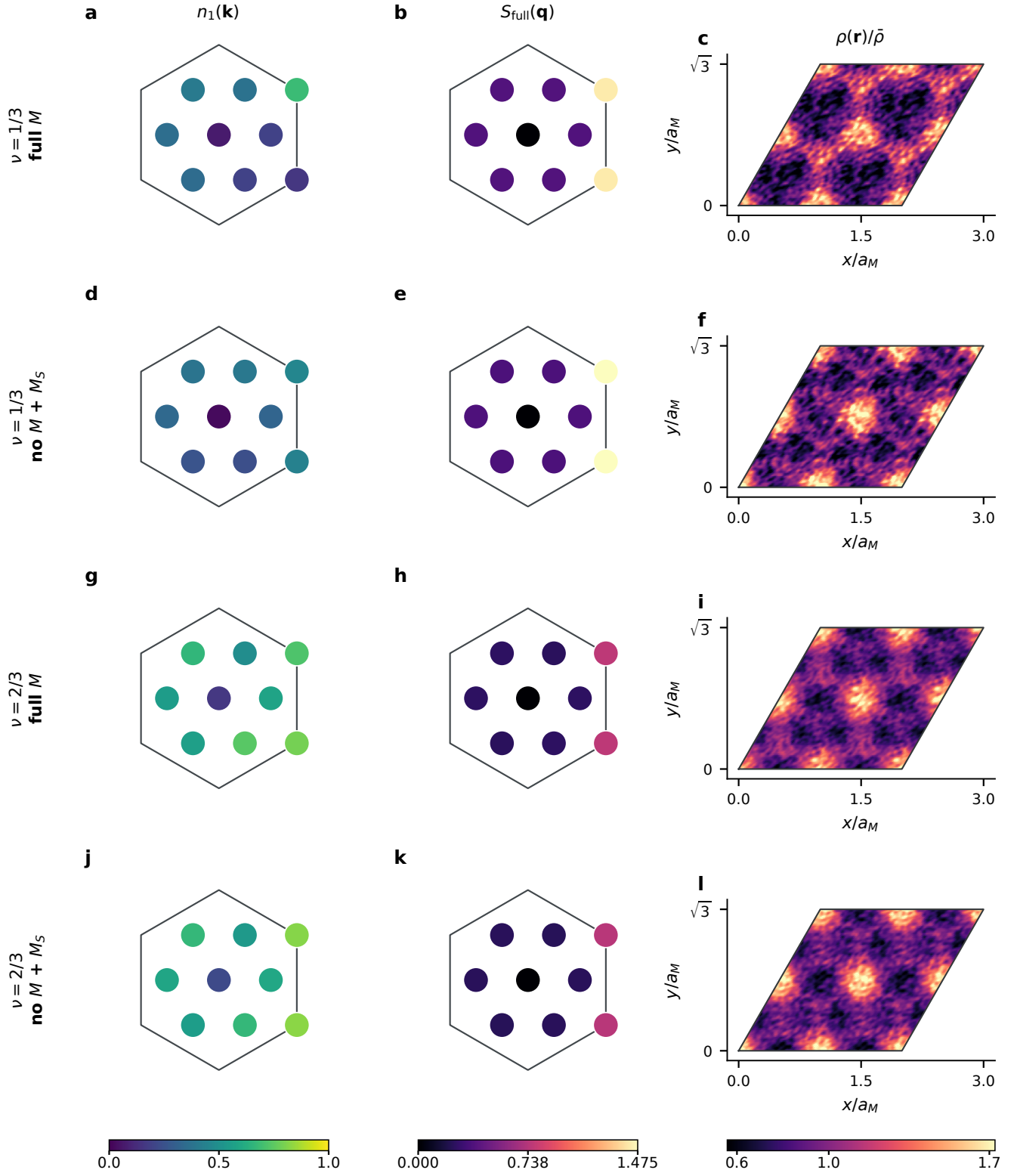
Figure 8: Full- M and \nu 3 no- M + M_S observables. The first two rows are \nu = 1/3 and the last two are \nu = 2/3 ; at each filling full M is followed by no M + M_S . Columns show bare-band-1 momentum occupation, the full static structure factor, and folded charge density. The \nu 3 no- M panels use the newly evaluated 4,128-configuration final ensembles.
