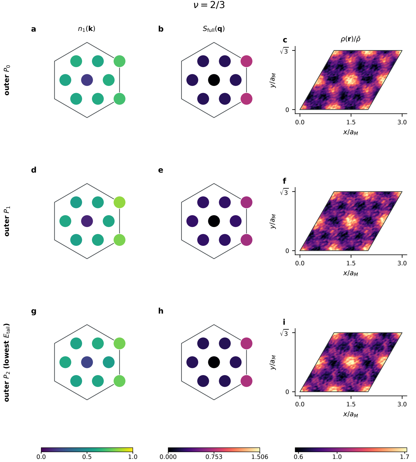
Figure 10: \nu = 2/3 outer-sector observables from final training samples. Rows are P_0, P_1, P_2 and columns use the same definitions and global color limits as Fig. 9. All panels use 4,128 configurations and 16 jointly batched auxiliary replacements per configuration. The three sectors are shown separately because both their band populations and two-body structure factors differ beyond a simple identical-map interpretation. The P_2 row is marked as the lowest final-ten-energy sector.
