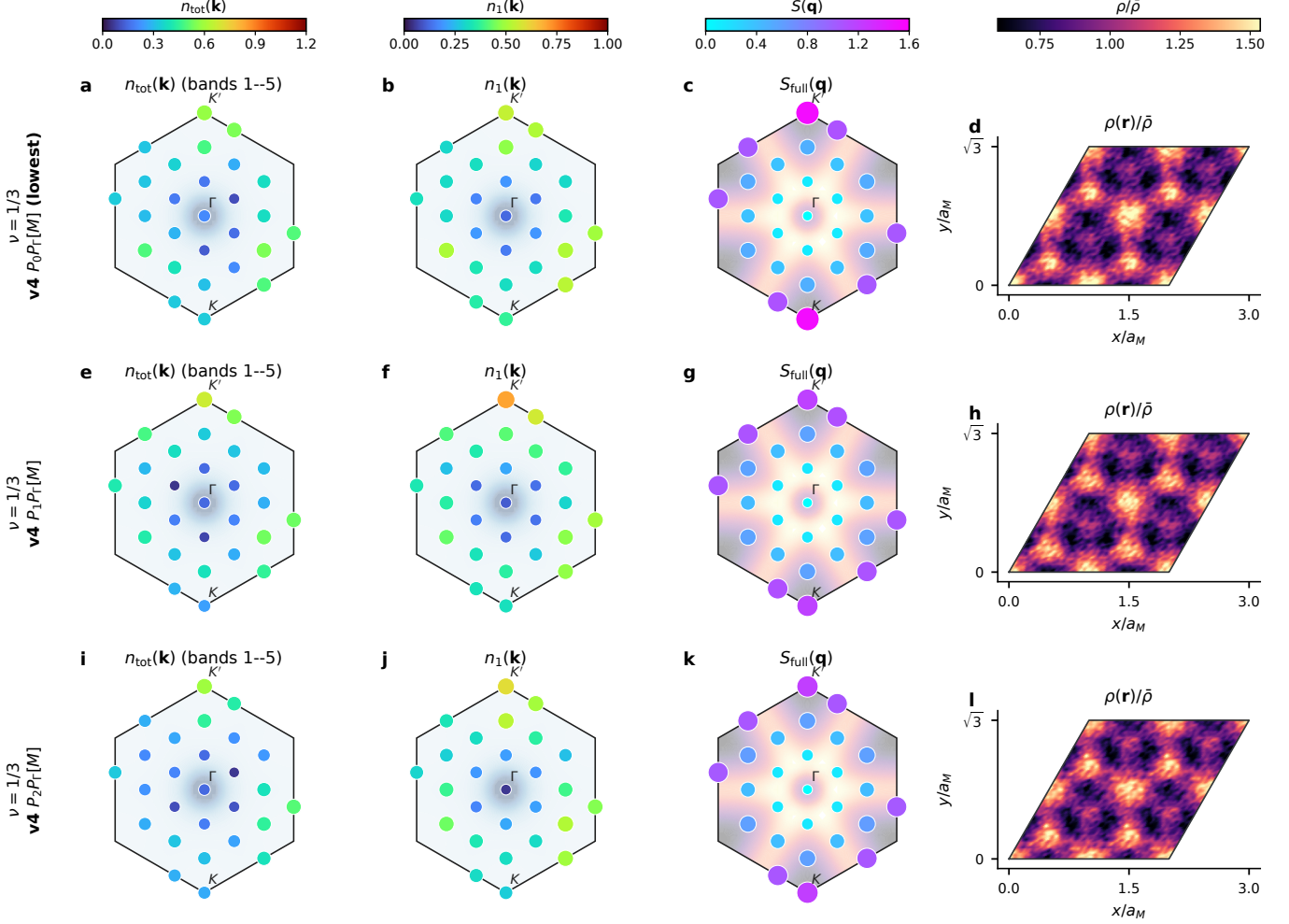
Figure 9: Twenty-seven-cell \nu = 1/3 outer-sector observables. Rows are the complete-wavefunction projectors P_0, P_1, P_2 ; the lowest final-ten branch is marked directly. Columns and all momentum-observable rendering conventions match Fig. 8 and the ED reference in Fig. 3. Shared color limits permit a direct visual comparison without sector-by-sector rescaling.
