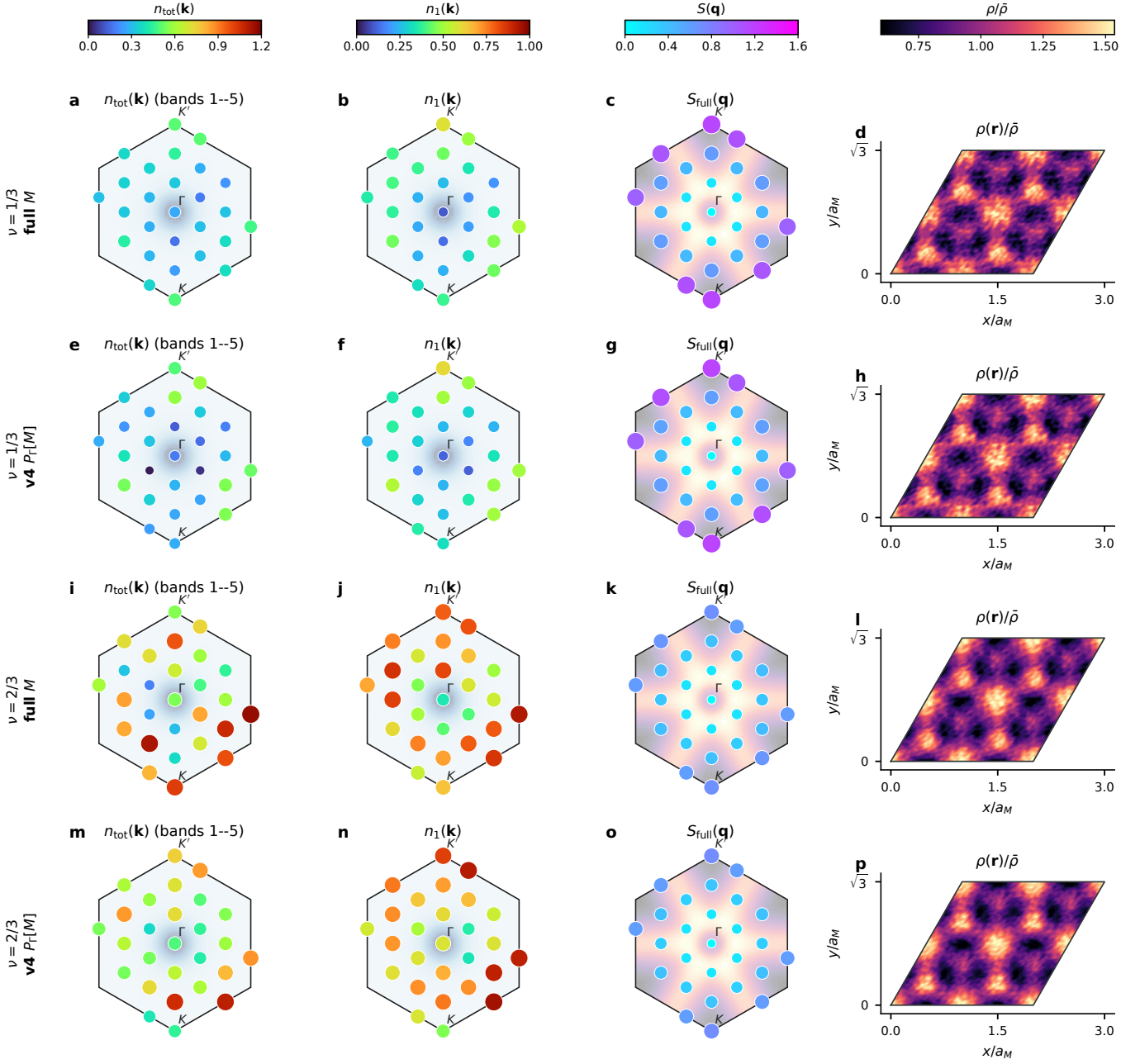
Figure 8: Twenty-seven-cell full- M and P_T[M] observables. Rows compare both ansatzes at \nu = 1/3 and 2/3 . Columns show the Bloch-projected occupation summed over bands 1–5, the band-1 occupation conditionally normalized to N_e , the full static structure factor transformed from the real-space density-pair correlation, and folded charge density. Both momentum panels and the main S(\mathbf{q}) panel use exactly the 27 physical ED momentum vectors. A directly evaluated 37-vector, C_6 -closed grid is retained only for boundary rotation audits. No observable is C_3 averaged, and no ED momentum profile enters the first-band normalization. All values use the saved final 4,128-walker training ensembles without a separate validation chain.
