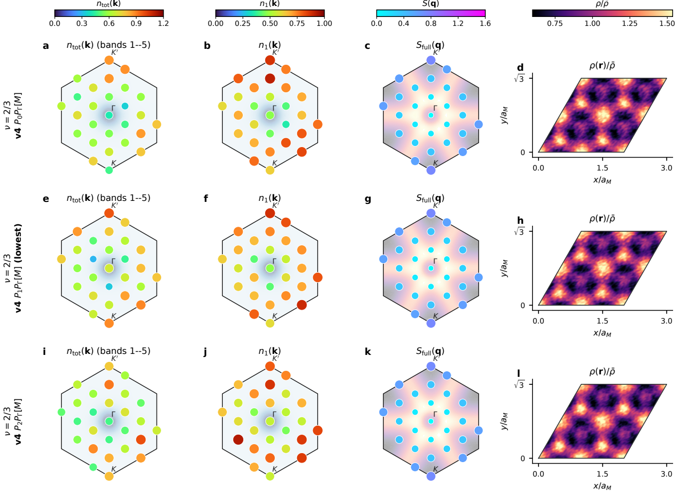
Figure 10: Twenty-seven-cell \nu = 2/3 outer-sector observables. Rows are P_0, P_1, P_2 and columns use the same definitions, color limits and marker rules as Fig. 9. The nearly degenerate final-ten m = 1, 2 energies are not by themselves evidence of a converged three-state manifold.
