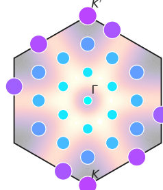
g S_{\text{full}}(\mathbf{q})
