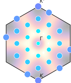
o S_{\text{full}}(\mathbf{q})
