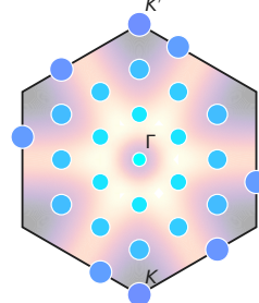
k S_{\text{full}}(\mathbf{q})
