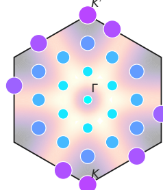
c S_{\text{full}}(\mathbf{q})
