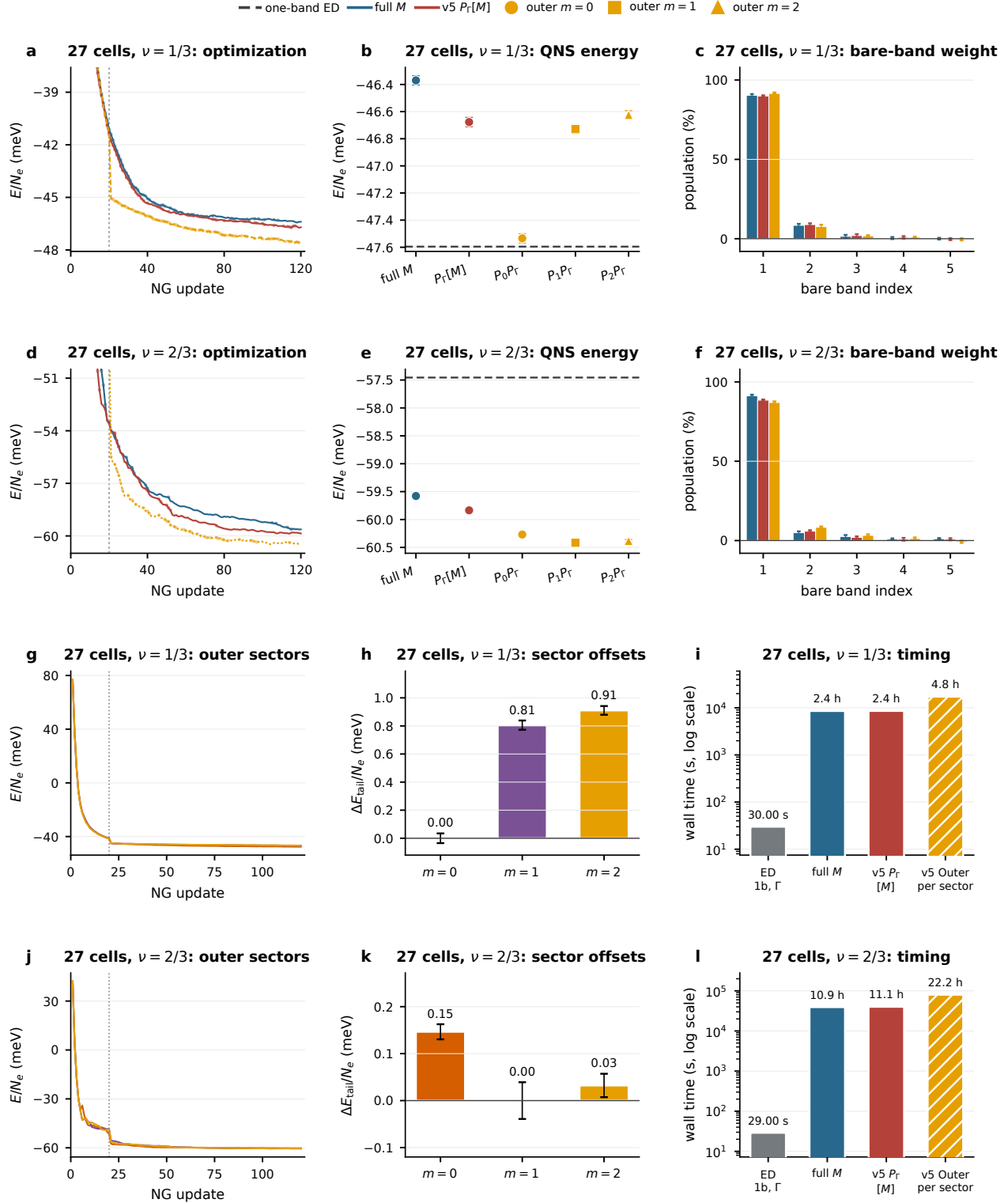
Figure 7: Twenty-seven-cell QNS summary. The layout follows Fig. 6. Since five-band 27-cell ED is unavailable, the energy panels use full M , P_r[M] and P_m P_r[M] as categorical abscissa labels; the one-band 27-cell ED energy is a dashed horizontal reference. All three outer-energy markers are yellow, with circle, square and triangle denoting m = 0, 1, 2 ; the selected outer-state band bars use the same yellow. Rows three and four resolve the three outer sectors and report measured training times. The hatched outer cost is the complete two-GPU critical path divided by the three resulting candidate states.
