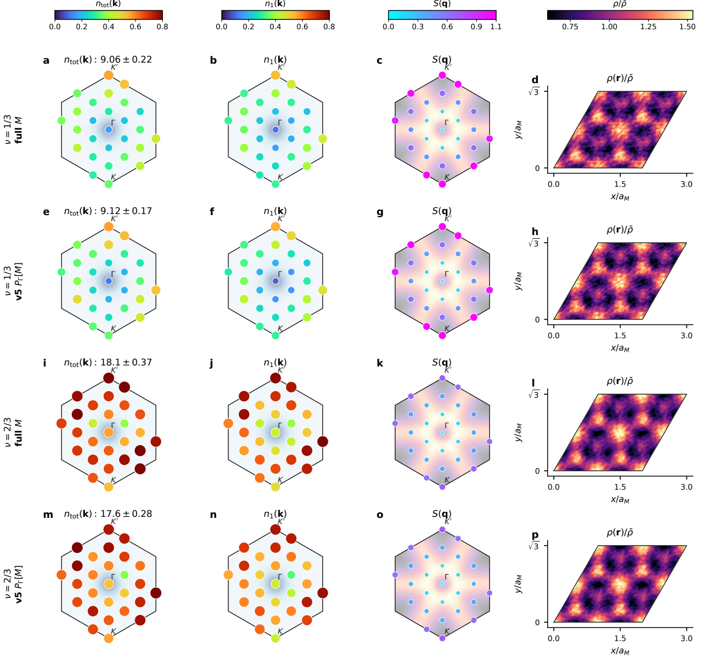
Figure 8: Twenty-seven-cell full- M and P_T[M] observables. Rows compare both ansatzes at \nu = 1/3 and 2/3 . Columns show n_{\text{tot}}(\mathbf{k}) , the band-1 occupation, the full static structure factor transformed from the real-space density-pair correlation, and folded charge density. The n_{\text{tot}} distribution is the raw Bloch-projected sum over bands 1–5; its 27-value trace and eight-block SEM are printed in the panel title as T_5 \pm \sigma_{T_5} , with respectively three and two significant digits. The band-1 panel shows the unrescaled physical projection, whose sum is N_e W_1 . The two momentum panels use the 27 ED Bloch vectors, and S(\mathbf{q}) uses those same 27 displayed vectors as literal Fourier momenta. For direct comparison, both occupation color ranges are fixed to [0, 0.8] and the S(\mathbf{q}) range to [0, 1.1] , matching Fig. 3; QNS values above them saturate at the top color rather than expanding the scale, while the marker area in all three momentum panels continues to grow with the stored value. In the occupation panels, \mathbf{k} is evaluated directly at the drawn first-BZ point and \mathbf{G} occurs only inside the Bloch plane-wave expansion. Each n_{\text{tot}} panel title gives its unnormalized five-band trace \sum_{\mathbf{k}} \tilde{n}_{\text{tot}} = T_5 and statistical uncertainty. Neither occupation is trace-normalized, no observable is C_3 averaged, and no ED momentum profile enters the postprocessing. All occupations use the saved final 4,128-walker training ensembles and 128 auxiliary coordinates per walker. The S(\mathbf{q}) and density columns use 20,640 configurations from five measurement-only steps of those same chains with the step-120 parameters frozen; no optimizer update is made.
