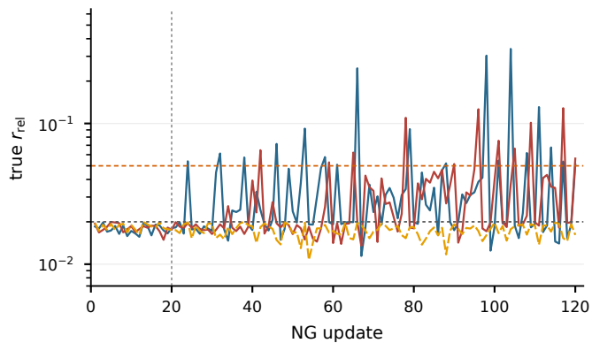
c 9 cells, \nu = 2/3
