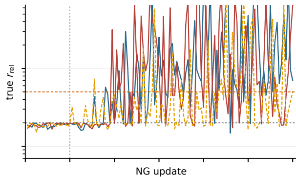
d 27 cells, \nu = 2/3
