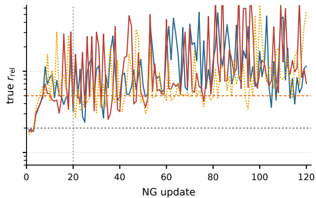
d 27 cells, \nu = 2/3
