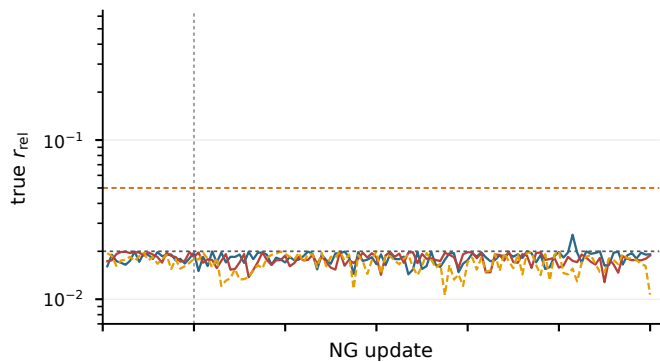
c 9 cells, \nu = 2/3
