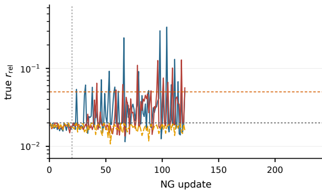
c 9 cells, \nu = 2/3
