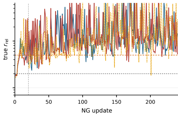
d 27 cells, \nu = 2/3
