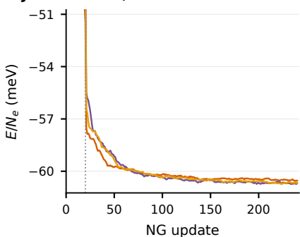
j 27 cells, \nu = 2/3 : outer sectors
