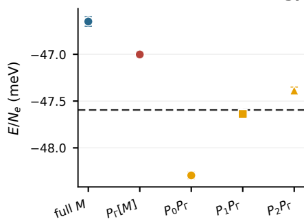
b 27 cells, \nu = 1/3 : QNS energy
