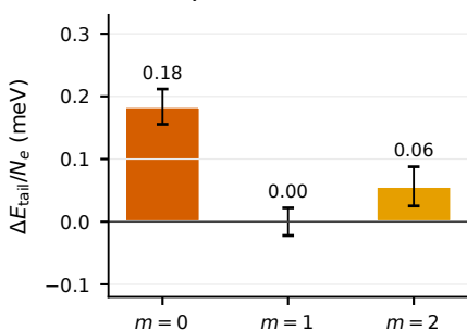
k 27 cells, \nu = 2/3 : sector offsets
