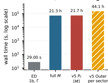
l 27 cells, \nu = 2/3 : timing
