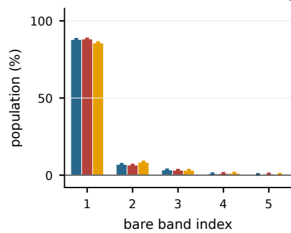
f 27 cells, \nu = 2/3 : bare-band weight
