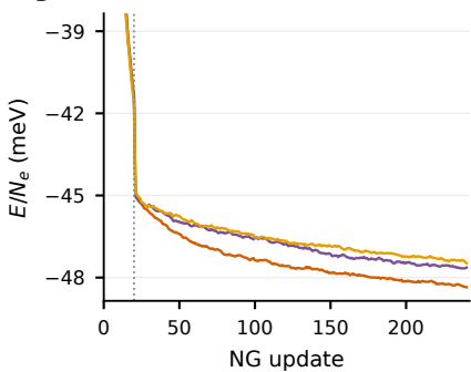
g 27 cells, \nu = 1/3 : outer sectors
