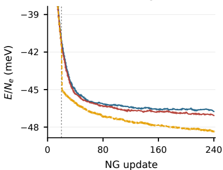
a 27 cells, \nu = 1/3 : optimization
