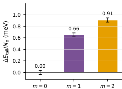
h 27 cells, \nu = 1/3 : sector offsets
