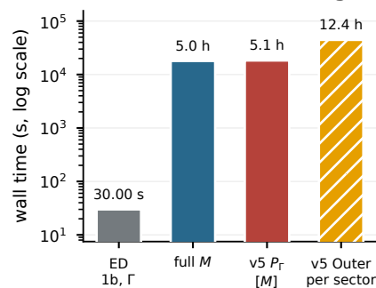
i 27 cells, \nu = 1/3 : timing
