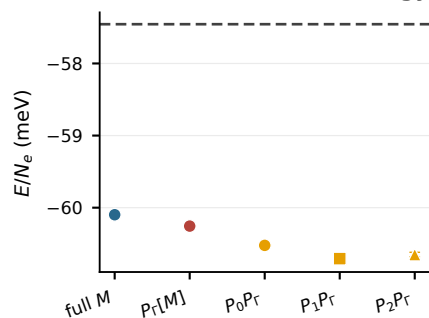
e 27 cells, \nu = 2/3 : QNS energy
