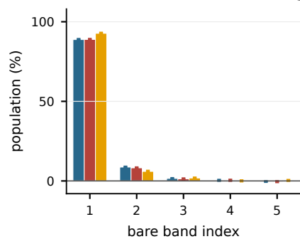
c 27 cells, \nu = 1/3 : bare-band weight
