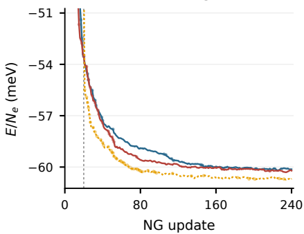
d 27 cells, \nu = 2/3 : optimization
