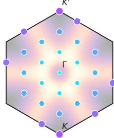
o S(\mathbf{q})
