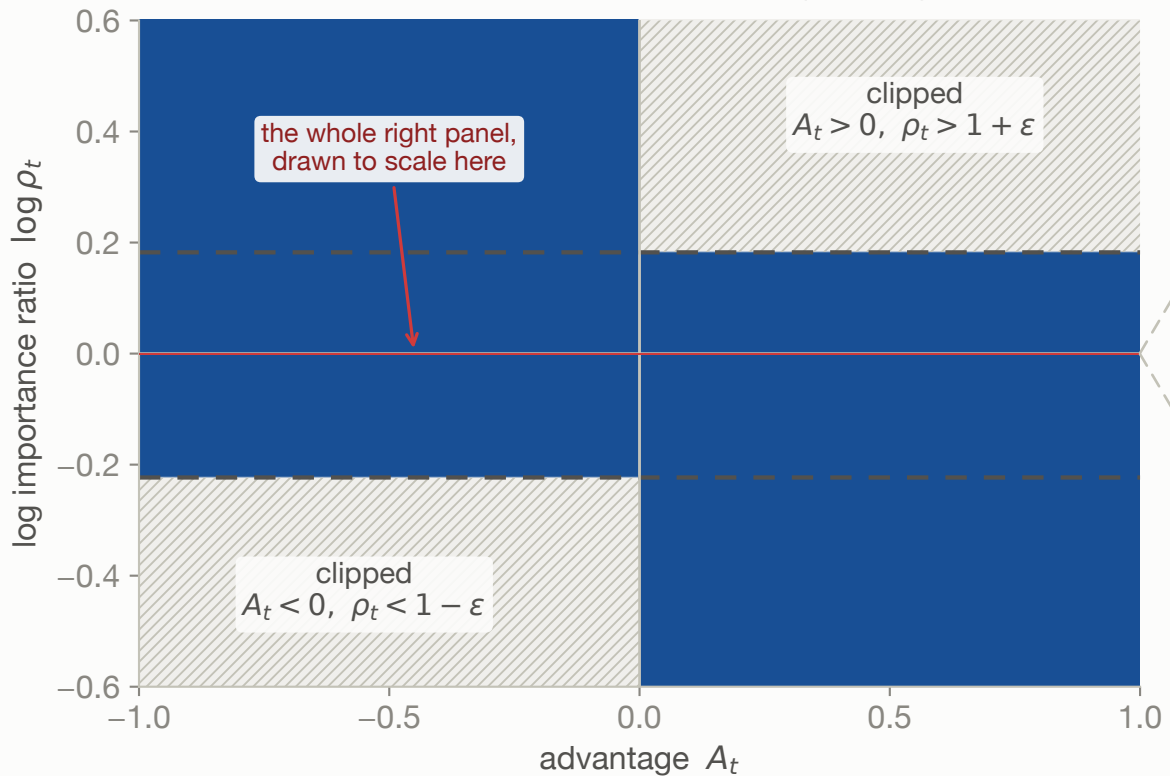
PPO / GRPO — token ratio ( \varepsilon = 0.2 )
