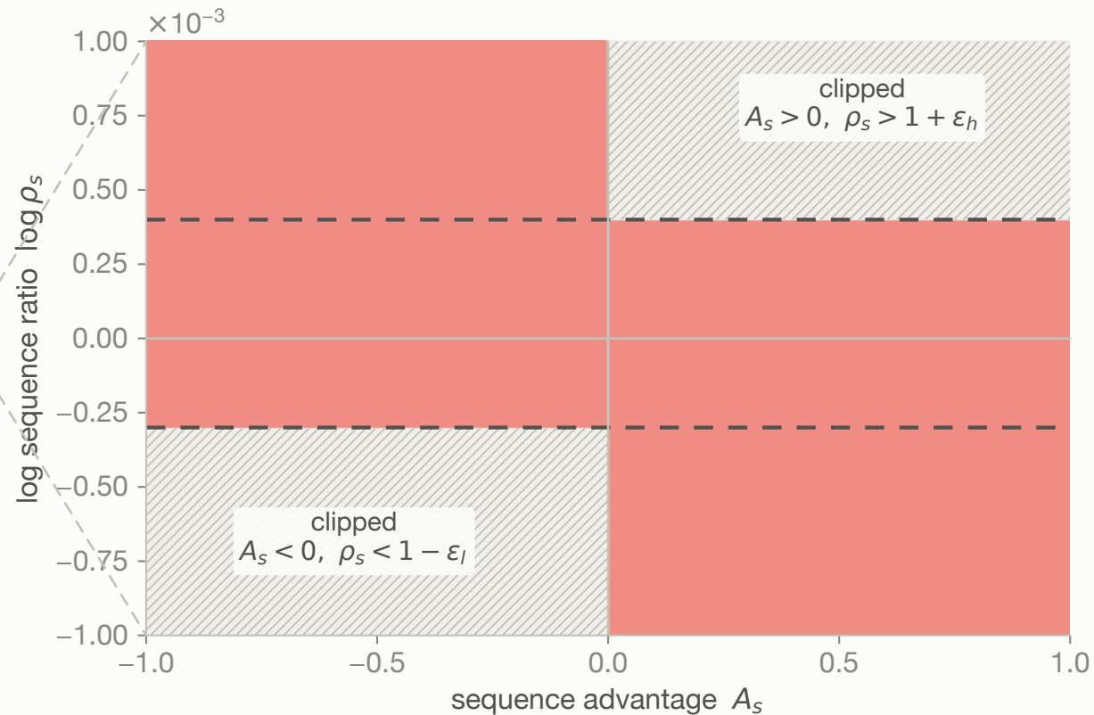
GSPO — sequence ratio ( \varepsilon_l = 3 \times 10^{-4}, \varepsilon_h = 4 \times 10^{-4} )
