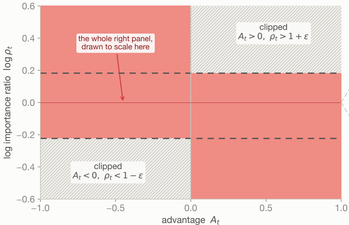
PPO / GRPO — token ratio ( \varepsilon = 0.2 )
