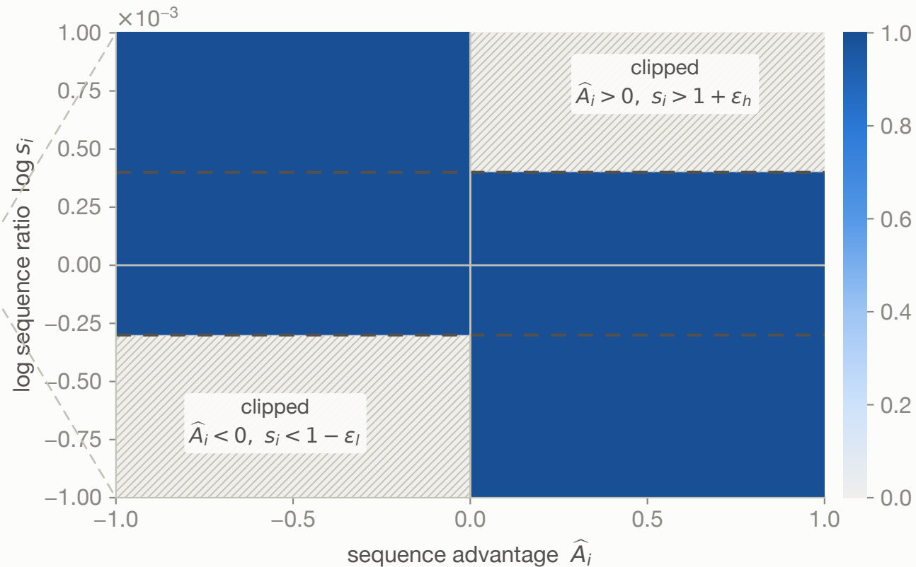
GSPO — sequence ratio ( \varepsilon_l = 3 \times 10^{-4}, \varepsilon_h = 4 \times 10^{-4} )
