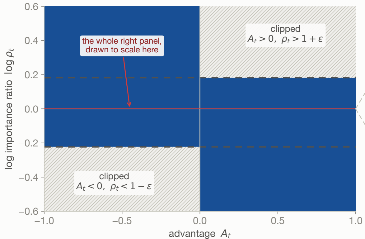
PPO / GRPO — token ratio ( \varepsilon = 0.2 )
