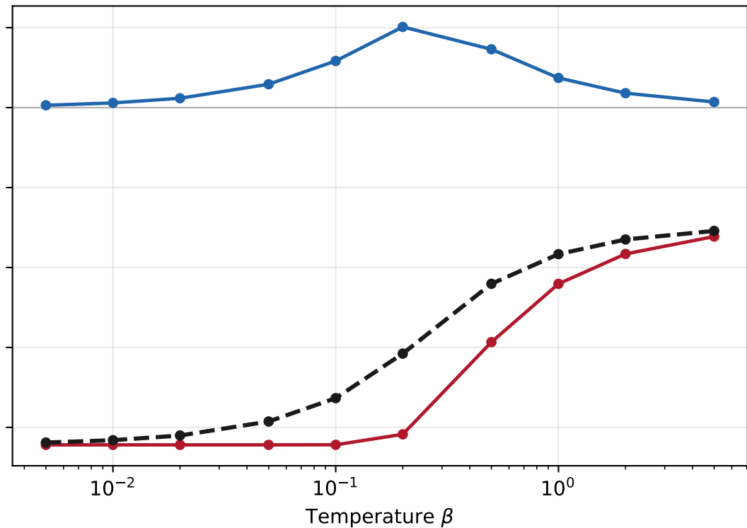
Length-normalized probability
