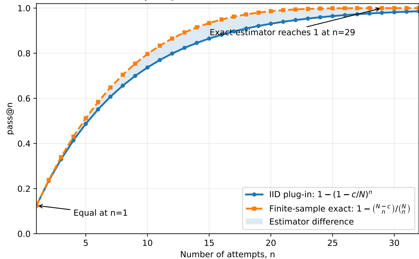
pass@n estimates for N=32, c=4
