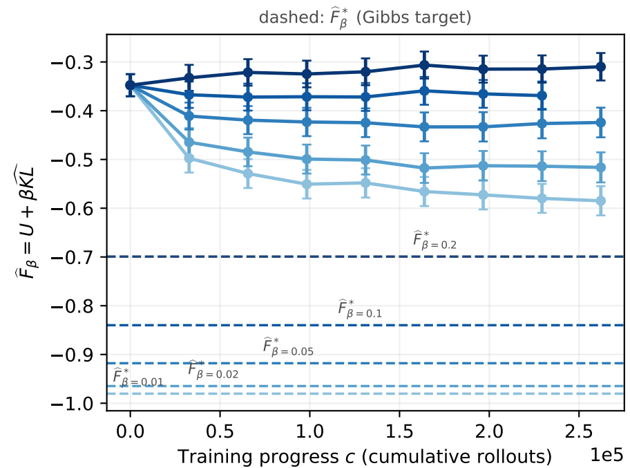
Free-energy decomposition across the KL penalty \beta : RLOO, G = 32 (held-out validation, paired checkpoints)
