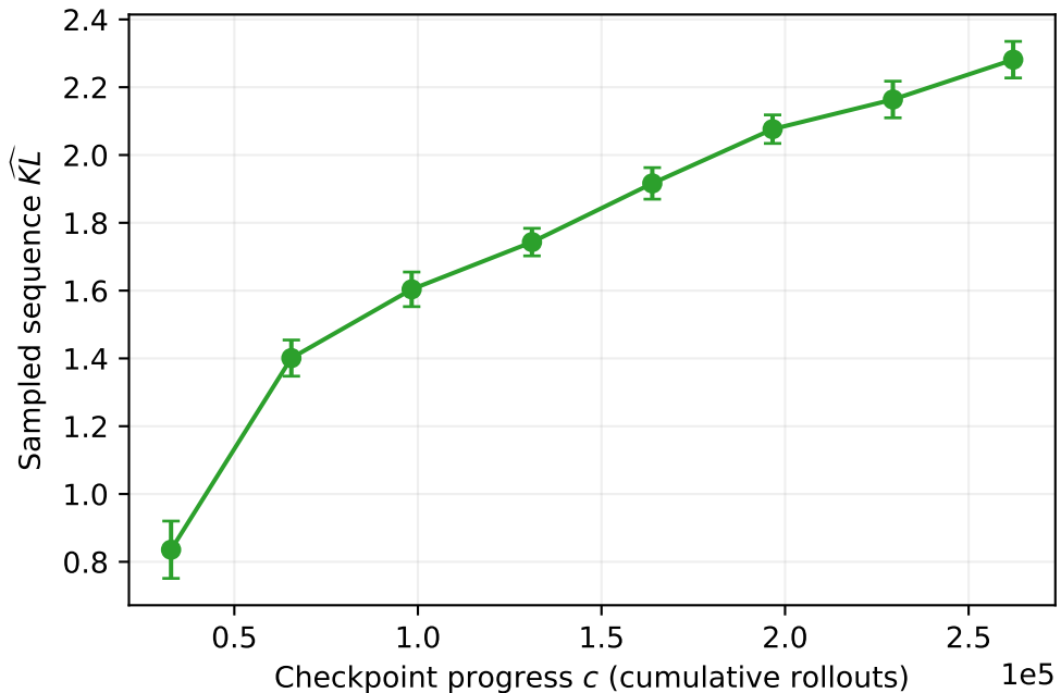
Between-checkpoint training blocks ( \beta = 0.05 , G = 32 )
