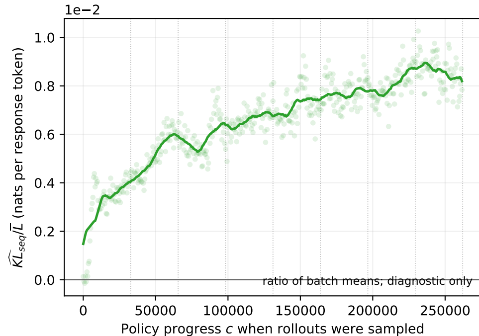
Length diagnostic for sampled KL: RLOO, \beta = 0.05 , G = 32 (token normalization is not a free energy)
