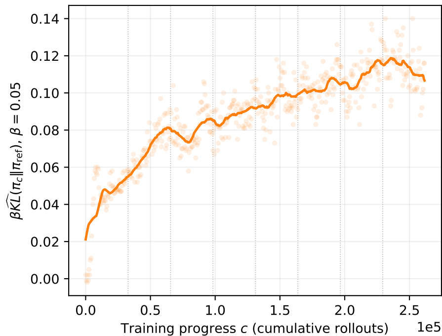
Free-energy decomposition: RLOO, \beta = 0.05 (on-policy training batches, 32-step rolling mean)
