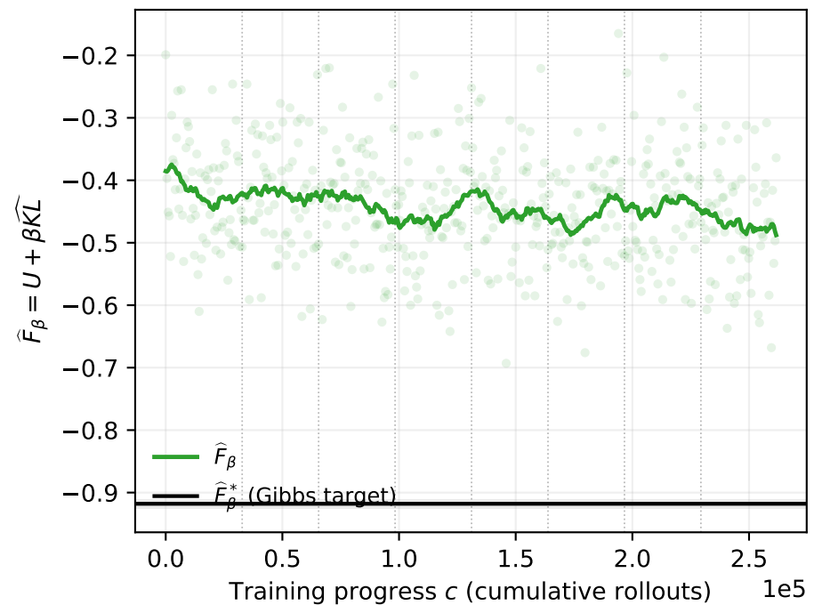
Free-energy decomposition: RLOO, \beta = 0.05 (on-policy training batches, 32-step rolling mean)
